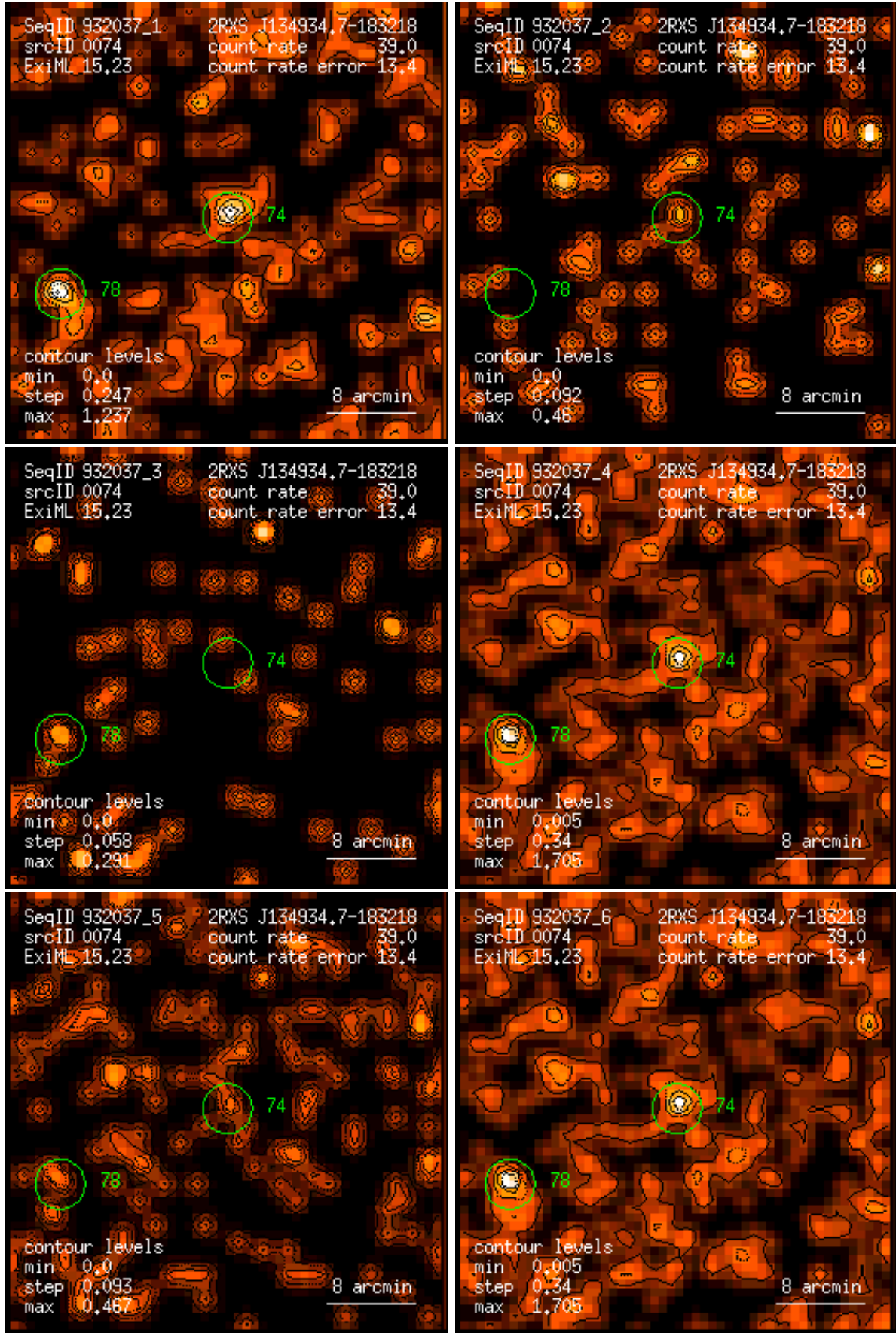
Figure 74: RASS 932037: detection 0074: band rate images, Gaussian filter: (1) PSPC channels 11 – 41, (2) 52 – 90, (3) 91 – 201, (4) 11 – 235, (5) 52 – 201, (6) 11 – 201. Broad band rates in counts/ks. Band rate contour levels in counts/ks/arcmin 2 .
