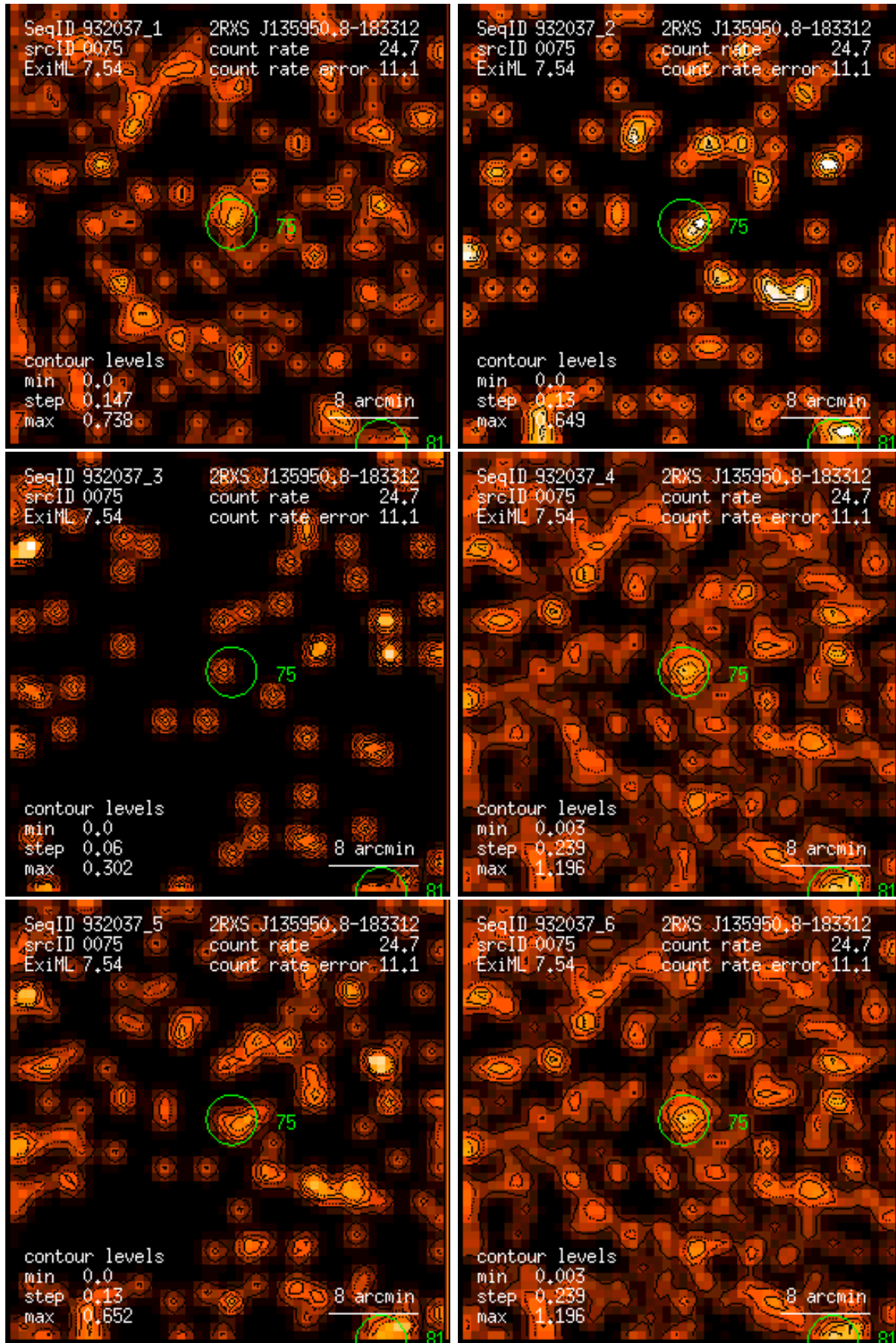
Figure 75: RASS 932037: detection 0075: band rate images, Gaussian filter: (1) PSPC channels 11 – 41, (2) 52 – 90, (3) 91 – 201, (4) 11 – 235, (5) 52 – 201, (6) 11 – 201. Broad band rates in counts/ks. Band rate contour levels in counts/ks/arcmin 2 .
