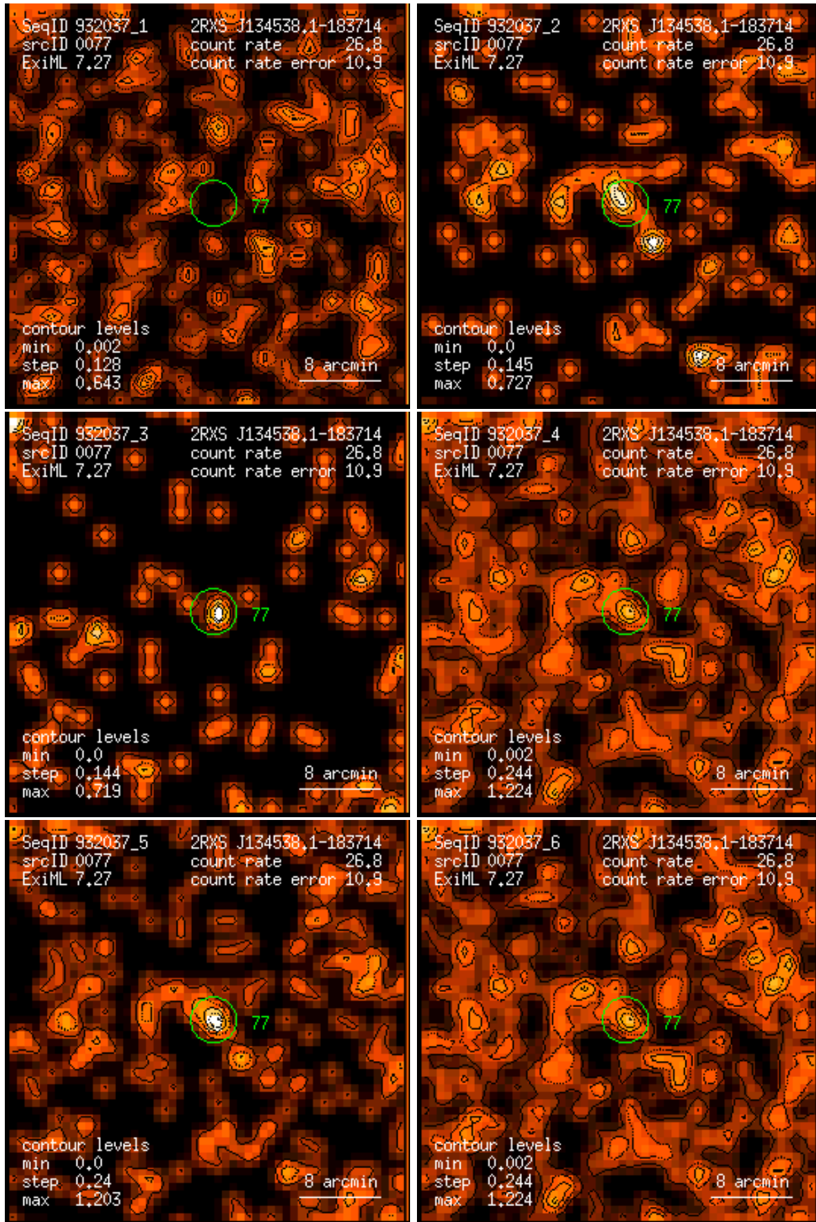
Figure 77: RASS 932037: detection 0077: band rate images, Gaussian filter: (1) PSPC channels 11 – 41, (2) 52 – 90, (3) 91 – 201, (4) 11 – 235, (5) 52 – 201, (6) 11 – 201. Broad band rates in counts/ks. Band rate contour levels in counts/ks/arcmin 2 .
