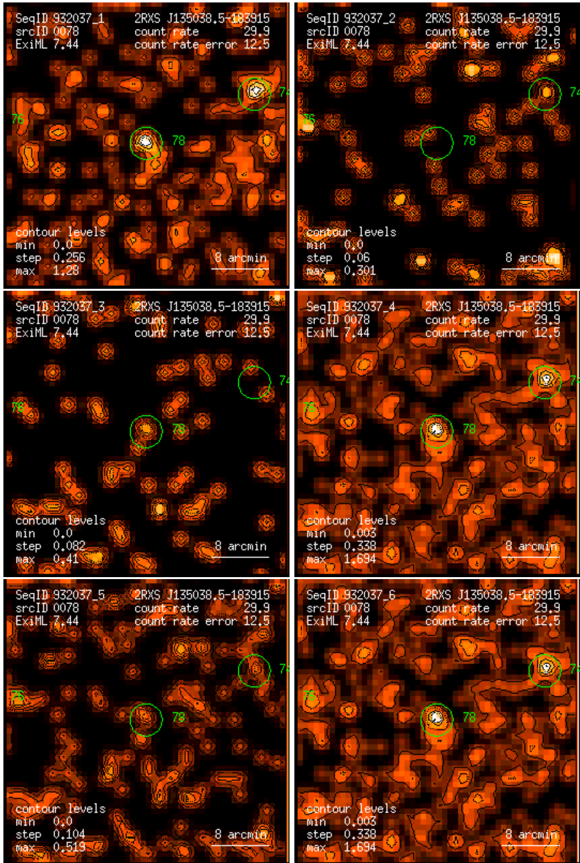
Figure 78: RASS 932037: detection 0078: band rate images, Gaussian filter: (1) PSPC channels 11 – 41, (2) 52 – 90, (3) 91 – 201, (4) 11 – 235, (5) 52 – 201, (6) 11 – 201. Broad band rates in counts/ks. Band rate contour levels in counts/ks/arcmin 2 .
