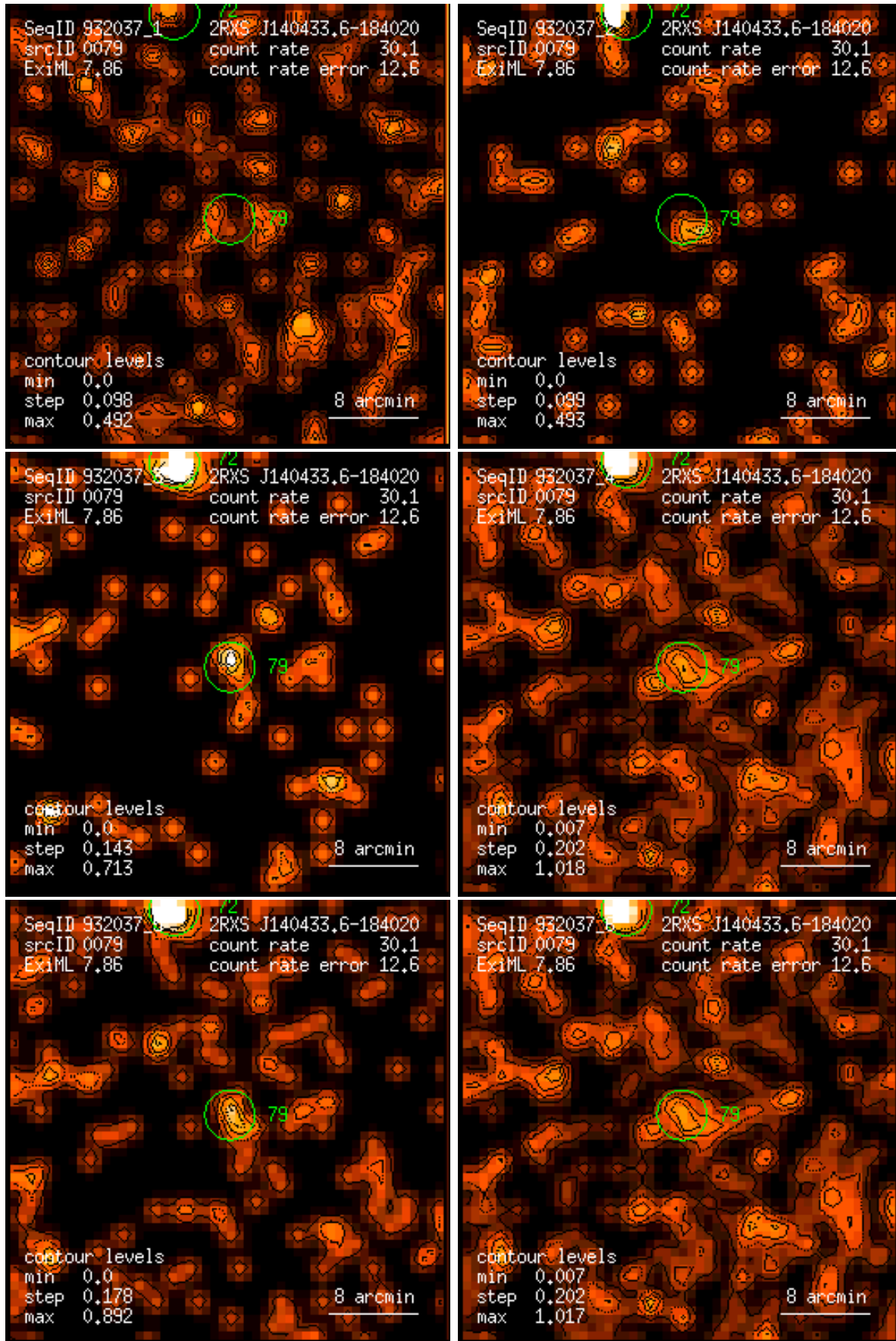
Figure 79: RASS 932037: detection 0079: band rate images, Gaussian filter: (1) PSPC channels 11 – 41, (2) 52 – 90, (3) 91 – 201, (4) 11 – 235, (5) 52 – 201, (6) 11 – 201. Broad band rates in counts/ks. Band rate contour levels in counts/ks/arcmin 2 .
