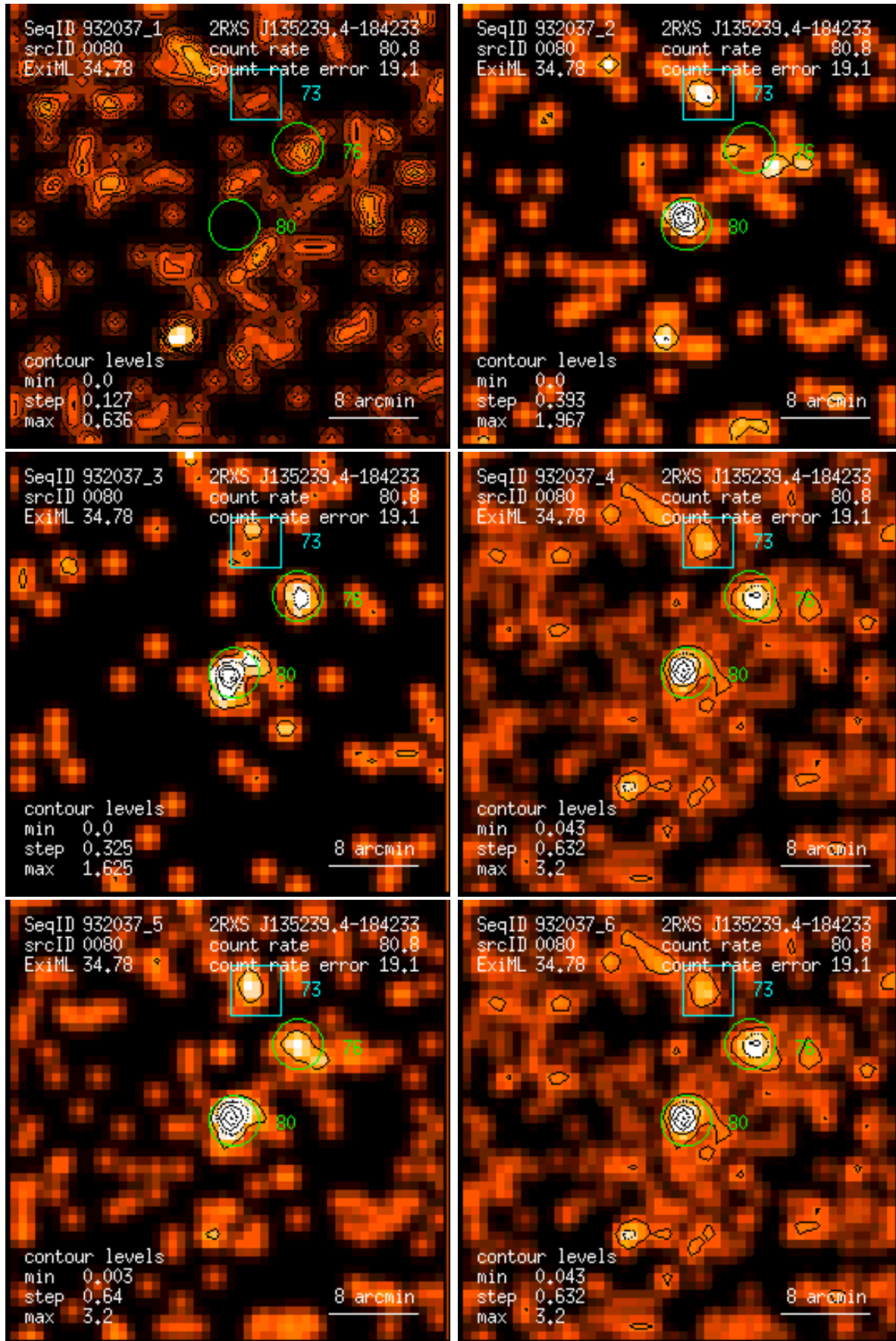
Figure 80: RASS 932037: detection 0080: band rate images, Gaussian filter: (1) PSPC channels 11 – 41, (2) 52 – 90, (3) 91 – 201, (4) 11 – 235, (5) 52 – 201, (6) 11 – 201. Broad band rates in counts/ks. Band rate contour levels in counts/ks/arcmin 2 .
