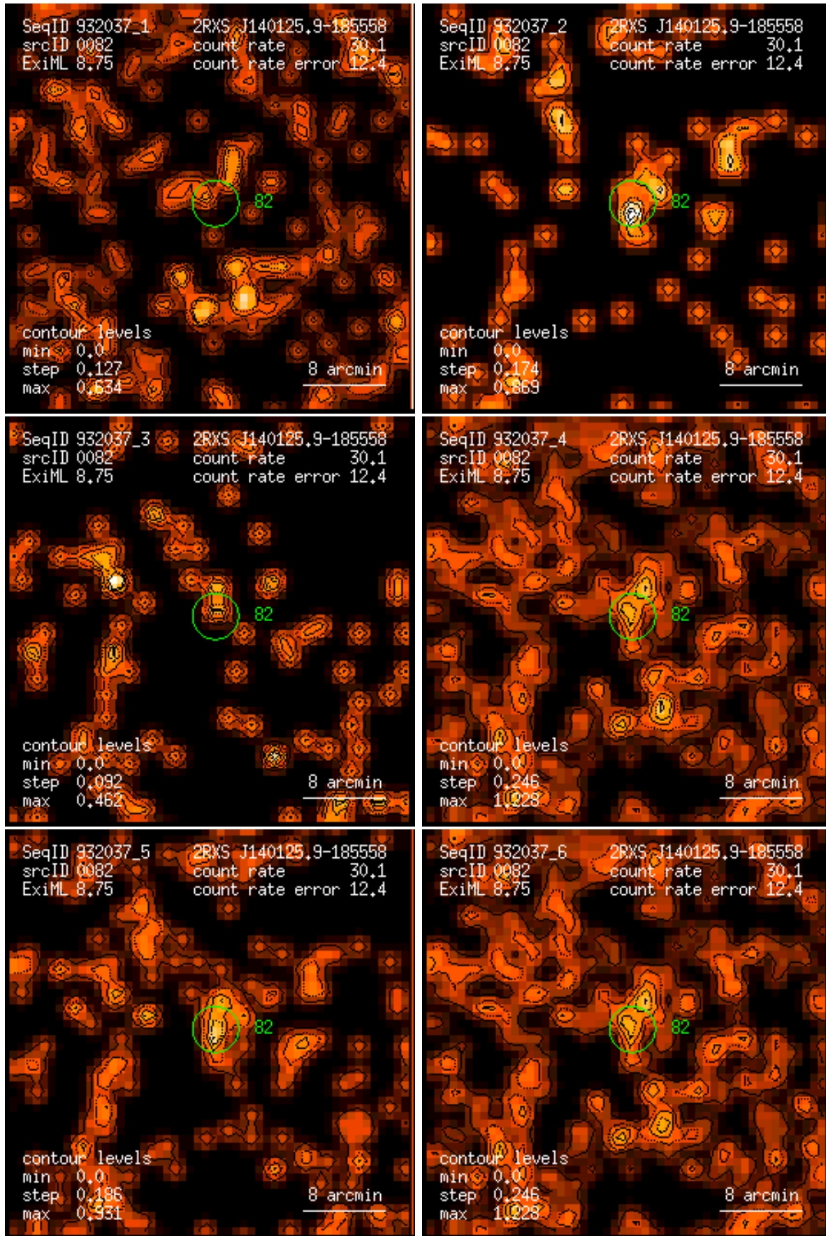
Figure 82: RASS 932037: detection 0082: band rate images, Gaussian filter: (1) PSPC channels 11 – 41, (2) 52 – 90, (3) 91 – 201, (4) 11 – 235, (5) 52 – 201, (6) 11 – 201. Broad band rates in counts/ks. Band rate contour levels in counts/ks/arcmin 2 .
