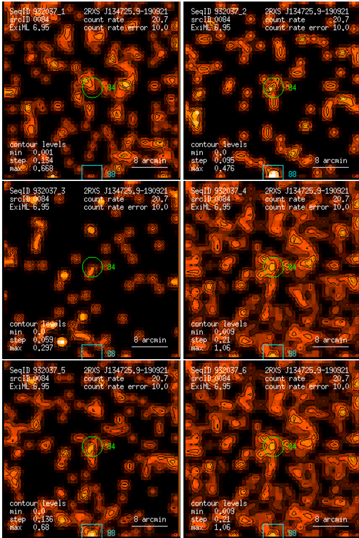
Figure 84: RASS 932037: detection 0084: band rate images, Gaussian filter: (1) PSPC channels 11 – 41, (2) 52 – 90, (3) 91 – 201, (4) 11 – 235, (5) 52 – 201, (6) 11 – 201. Broad band rates in counts/ks. Band rate contour levels in counts/ks/arcmin 2 .
