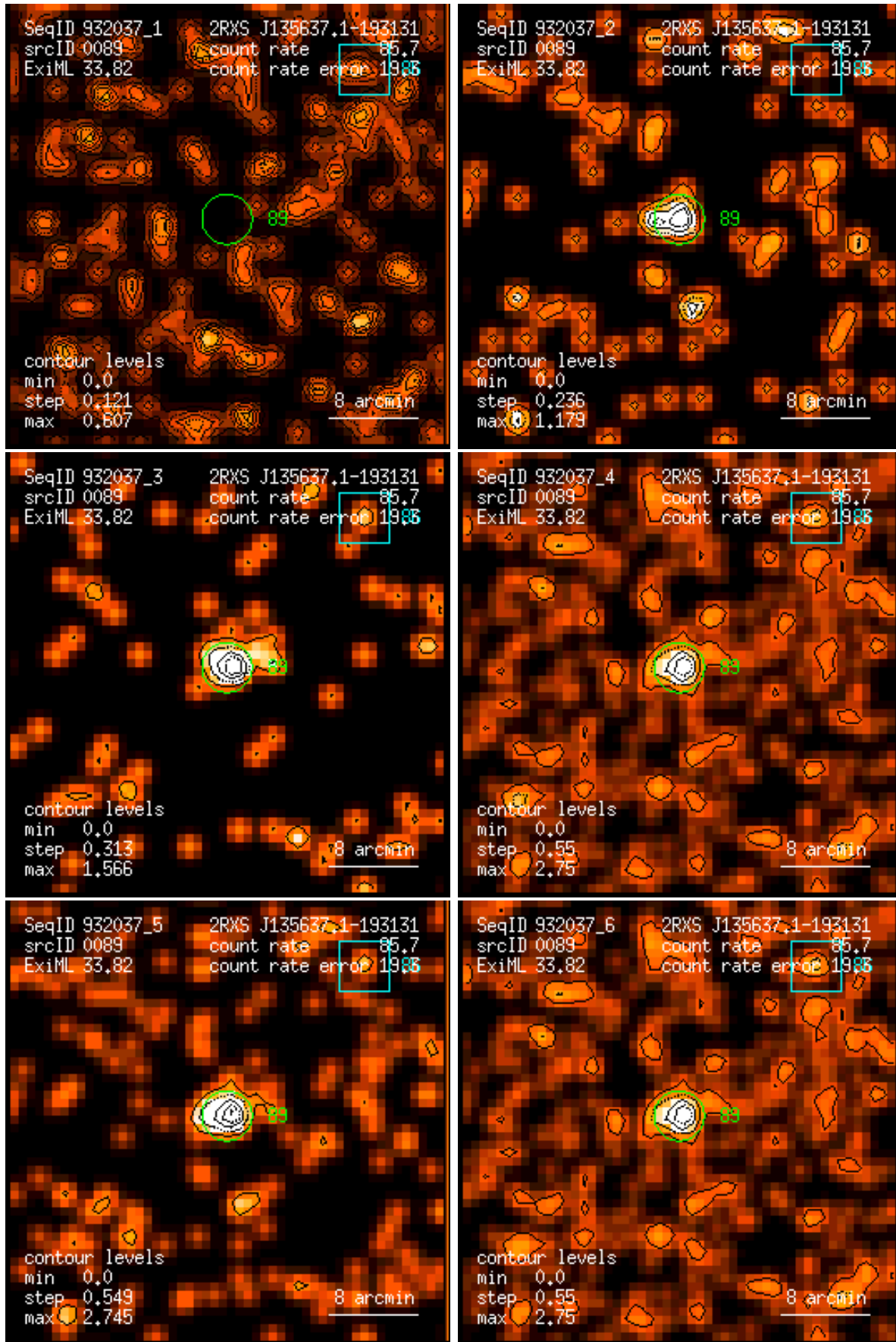
Figure 89: RASS 932037: detection 0089: band rate images, Gaussian filter: (1) PSPC channels 11 – 41, (2) 52 – 90, (3) 91 – 201, (4) 11 – 235, (5) 52 – 201, (6) 11 – 201. Broad band rates in counts/ks. Band rate contour levels in counts/ks/arcmin 2 .
