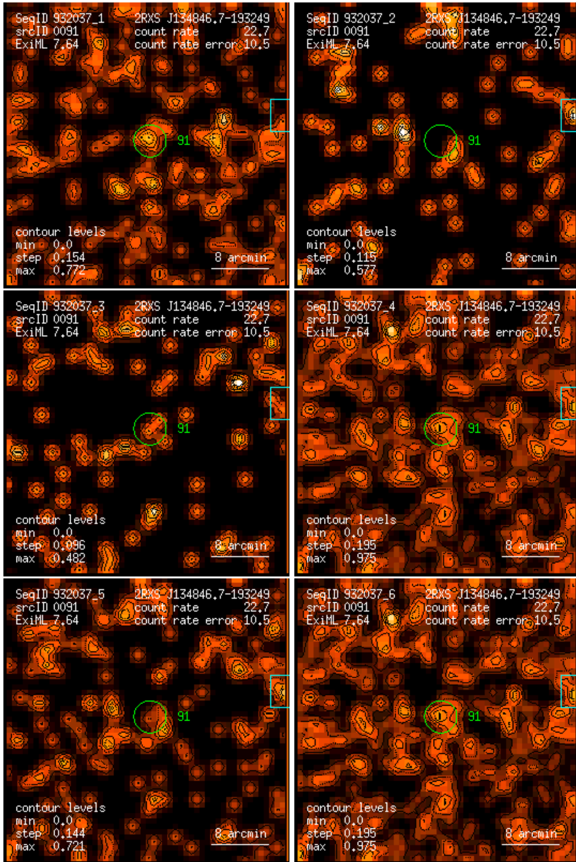
Figure 91: RASS 932037: detection 0091: band rate images, Gaussian filter: (1) PSPC channels 11 – 41, (2) 52 – 90, (3) 91 – 201, (4) 11 – 235, (5) 52 – 201, (6) 11 – 201. Broad band rates in counts/ks. Band rate contour levels in counts/ks/arcmin 2 .
