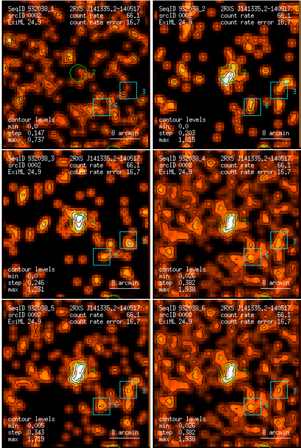
Figure 2: RASS 932038: detection 0002: band rate images, Gaussian filter: (1) PSPC channels 11 – 41, (2) 52 – 90, (3) 91 – 201, (4) 11 – 235, (5) 52 – 201, (6) 11 – 201. Broad band rates in counts/ks. Band rate contour levels in counts/ks/arcmin 2 .
