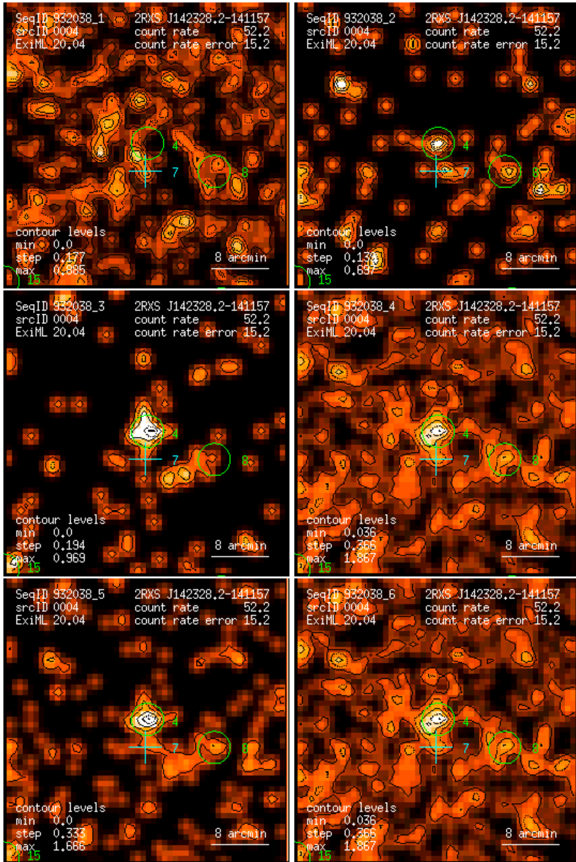
Figure 4: RASS 932038: detection 0004: band rate images, Gaussian filter: (1) PSPC channels 11 – 41, (2) 52 – 90, (3) 91 – 201, (4) 11 – 235, (5) 52 – 201, (6) 11 – 201. Broad band rates in counts/ks. Band rate contour levels in counts/ks/arcmin 2 .
