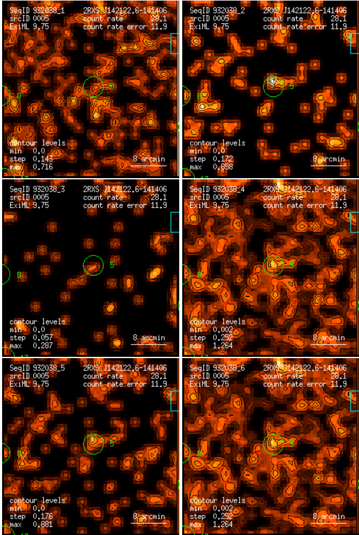
Figure 5: RASS 932038: detection 0005: band rate images, Gaussian filter: (1) PSPC channels 11 – 41, (2) 52 – 90, (3) 91 – 201, (4) 11 – 235, (5) 52 – 201, (6) 11 – 201. Broad band rates in counts/ks. Band rate contour levels in counts/ks/arcmin 2 .
