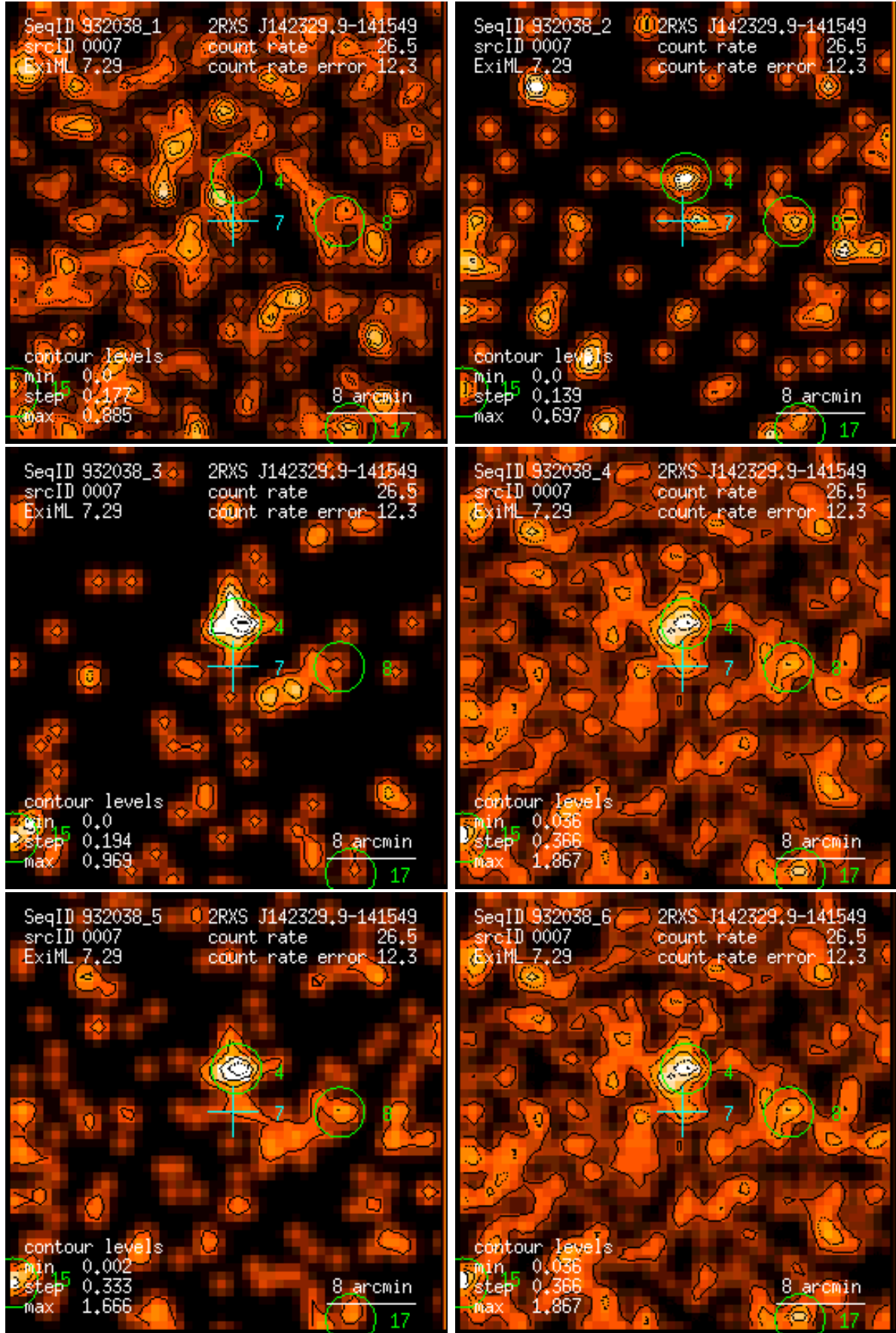
Figure 7: RASS 932038: detection 0007: band rate images, Gaussian filter: (1) PSPC channels 11 – 41, (2) 52 – 90, (3) 91 – 201, (4) 11 – 235, (5) 52 – 201, (6) 11 – 201. Broad band rates in counts/ks. Band rate contour levels in counts/ks/arcmin 2 .
