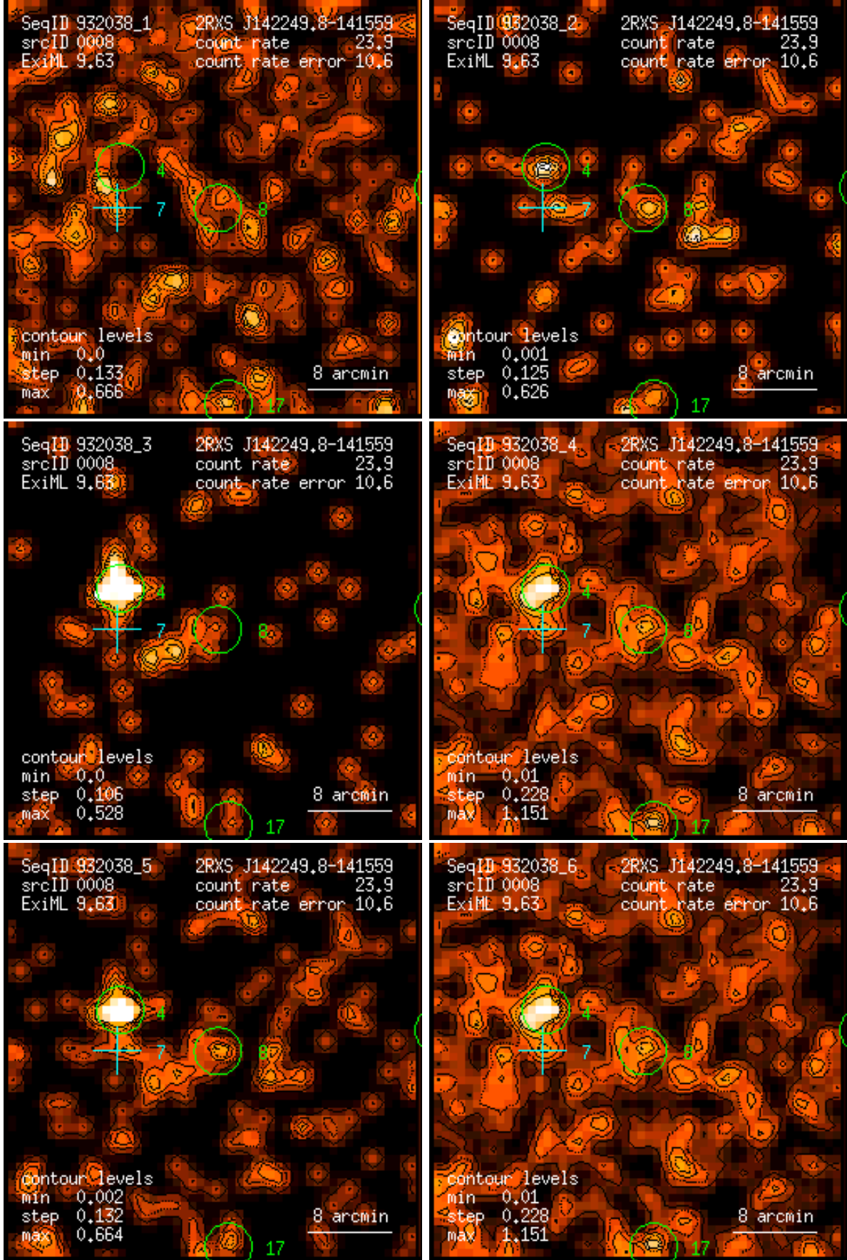
Figure 8: RASS 932038: detection 0008: band rate images, Gaussian filter: (1) PSPC channels 11 – 41, (2) 52 – 90, (3) 91 – 201, (4) 11 – 235, (5) 52 – 201, (6) 11 – 201. Broad band rates in counts/ks. Band rate contour levels in counts/ks/arcmin 2 .
