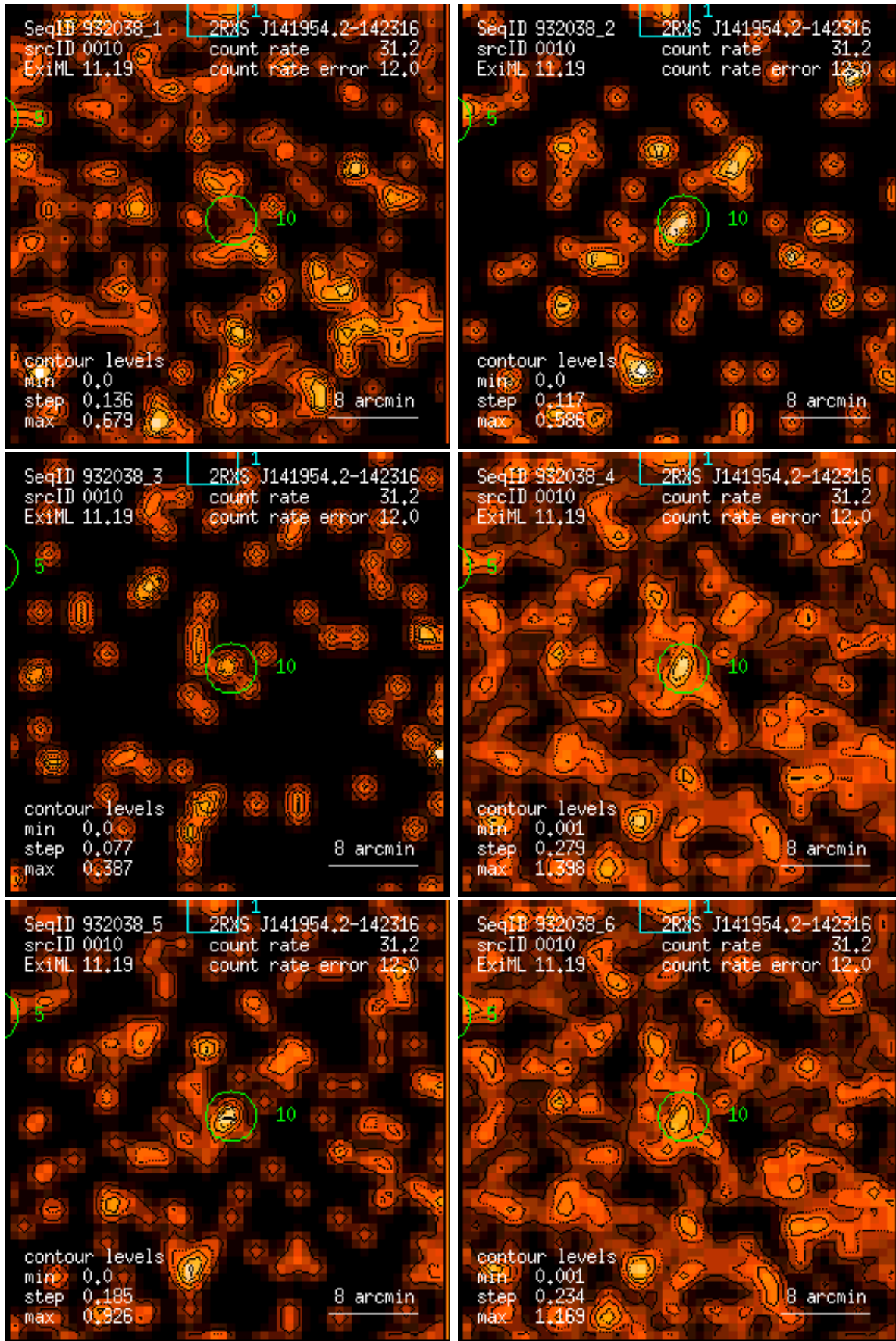
Figure 10: RASS 932038: detection 0010: band rate images, Gaussian filter: (1) PSPC channels 11 – 41, (2) 52 – 90, (3) 91 – 201, (4) 11 – 235, (5) 52 – 201, (6) 11 – 201. Broad band rates in counts/ks. Band rate contour levels in counts/ks/arcmin 2 .
