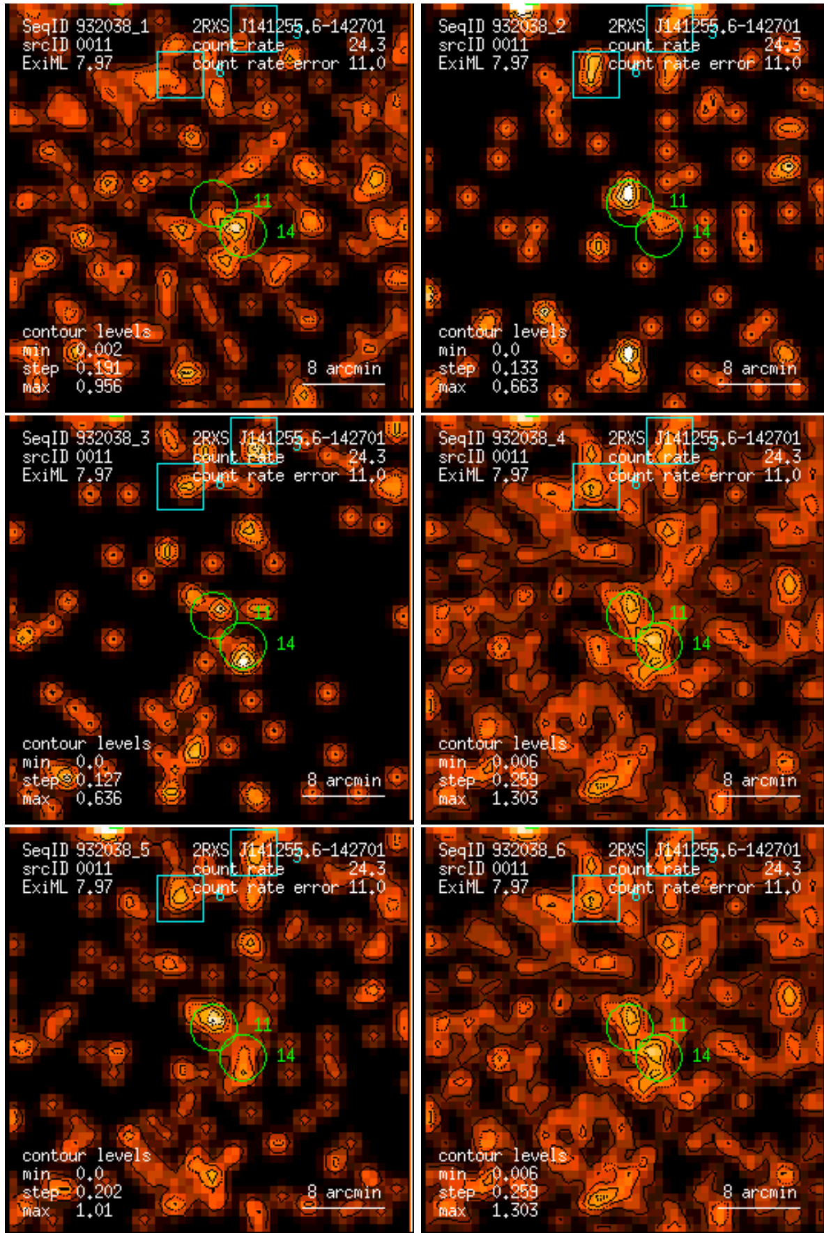
Figure 11: RASS 932038: detection 0011: band rate images, Gaussian filter: (1) PSPC channels 11 – 41, (2) 52 – 90, (3) 91 – 201, (4) 11 – 235, (5) 52 – 201, (6) 11 – 201. Broad band rates in counts/ks. Band rate contour levels in counts/ks/arcmin 2 .
