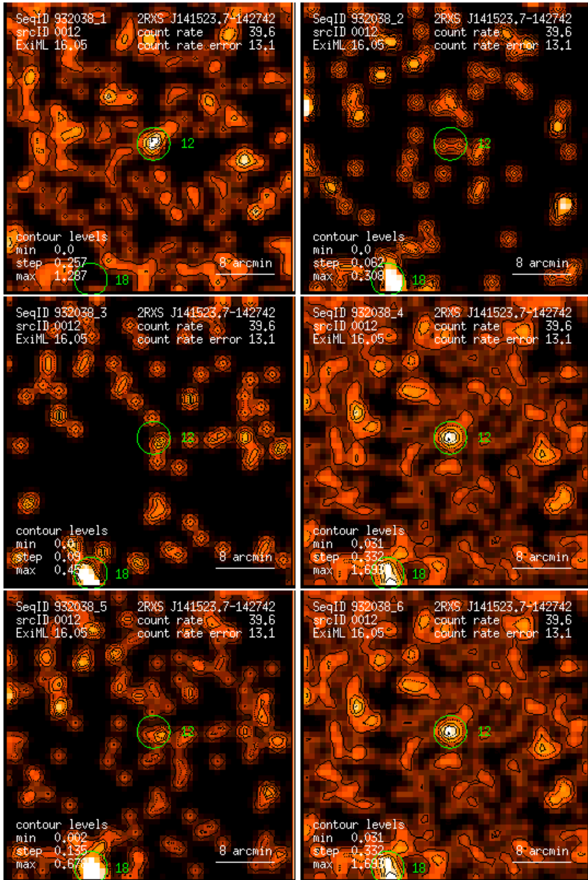
Figure 12: RASS 932038: detection 0012: band rate images, Gaussian filter: (1) PSPC channels 11 – 41, (2) 52 – 90, (3) 91 – 201, (4) 11 – 235, (5) 52 – 201, (6) 11 – 201. Broad band rates in counts/ks. Band rate contour levels in counts/ks/arcmin 2 .
