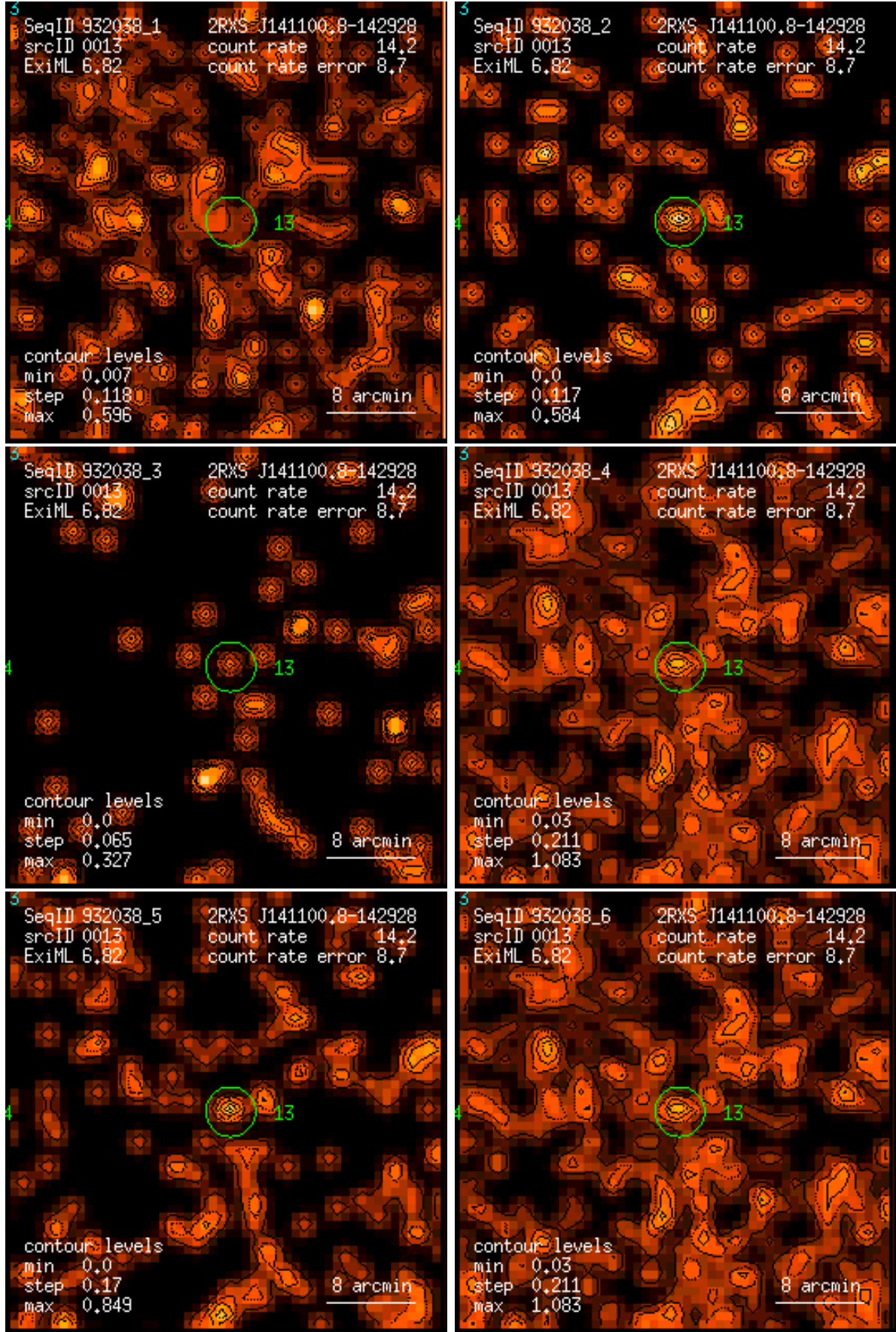
Figure 13: RASS 932038: detection 0013: band rate images, Gaussian filter: (1) PSPC channels 11 – 41, (2) 52 – 90, (3) 91 – 201, (4) 11 – 235, (5) 52 – 201, (6) 11 – 201. Broad band rates in counts/ks. Band rate contour levels in counts/ks/arcmin 2 .
