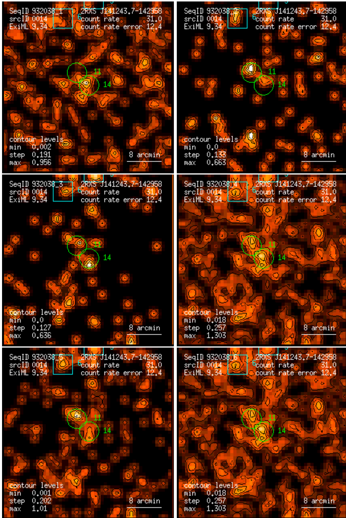
Figure 14: RASS 932038: detection 0014: band rate images, Gaussian filter: (1) PSPC channels 11 – 41, (2) 52 – 90, (3) 91 – 201, (4) 11 – 235, (5) 52 – 201, (6) 11 – 201. Broad band rates in counts/ks. Band rate contour levels in counts/ks/arcmin 2 .
