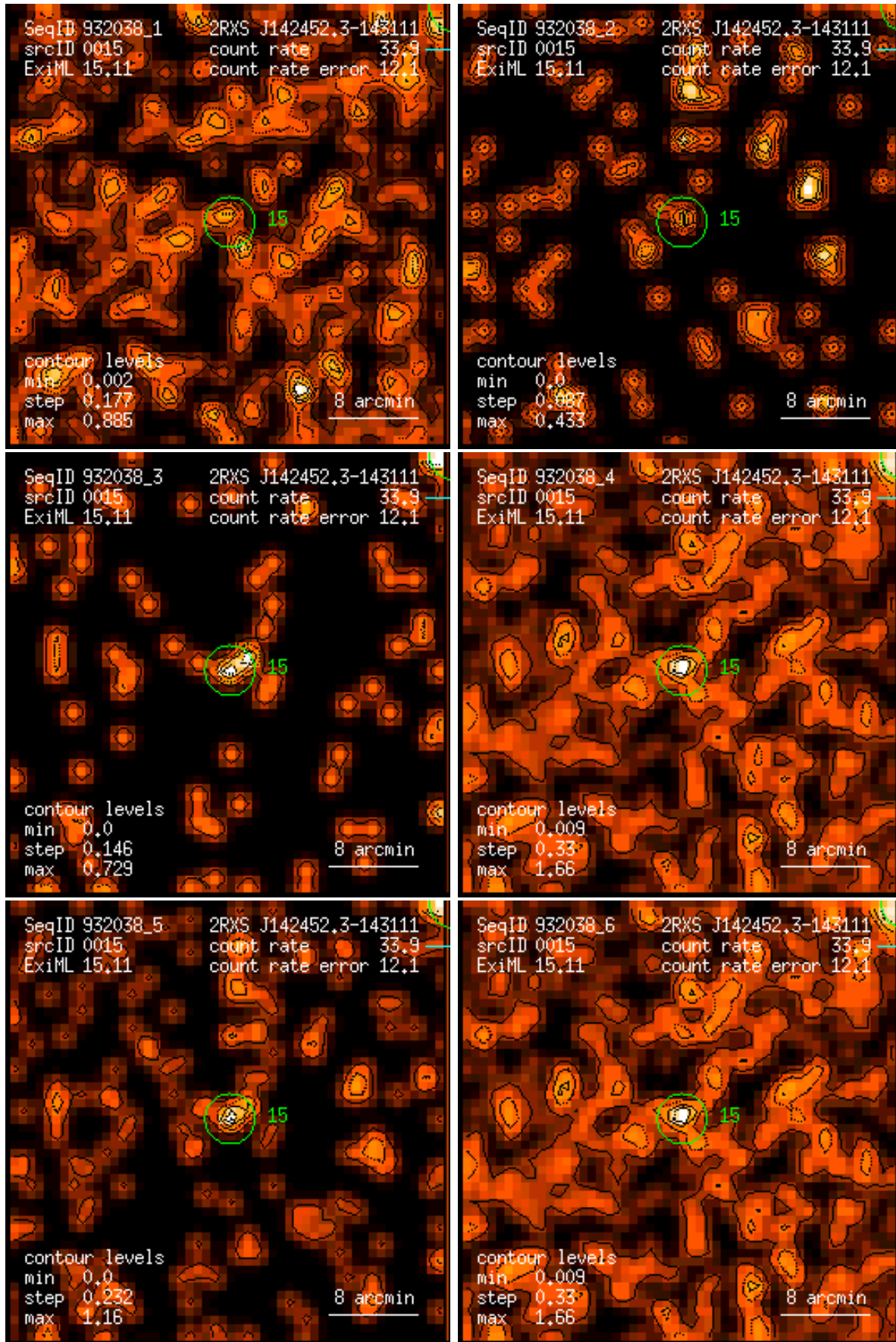
Figure 15: RASS 932038: detection 0015: band rate images, Gaussian filter: (1) PSPC channels 11 – 41, (2) 52 – 90, (3) 91 – 201, (4) 11 – 235, (5) 52 – 201, (6) 11 – 201. Broad band rates in counts/ks. Band rate contour levels in counts/ks/arcmin 2 .
