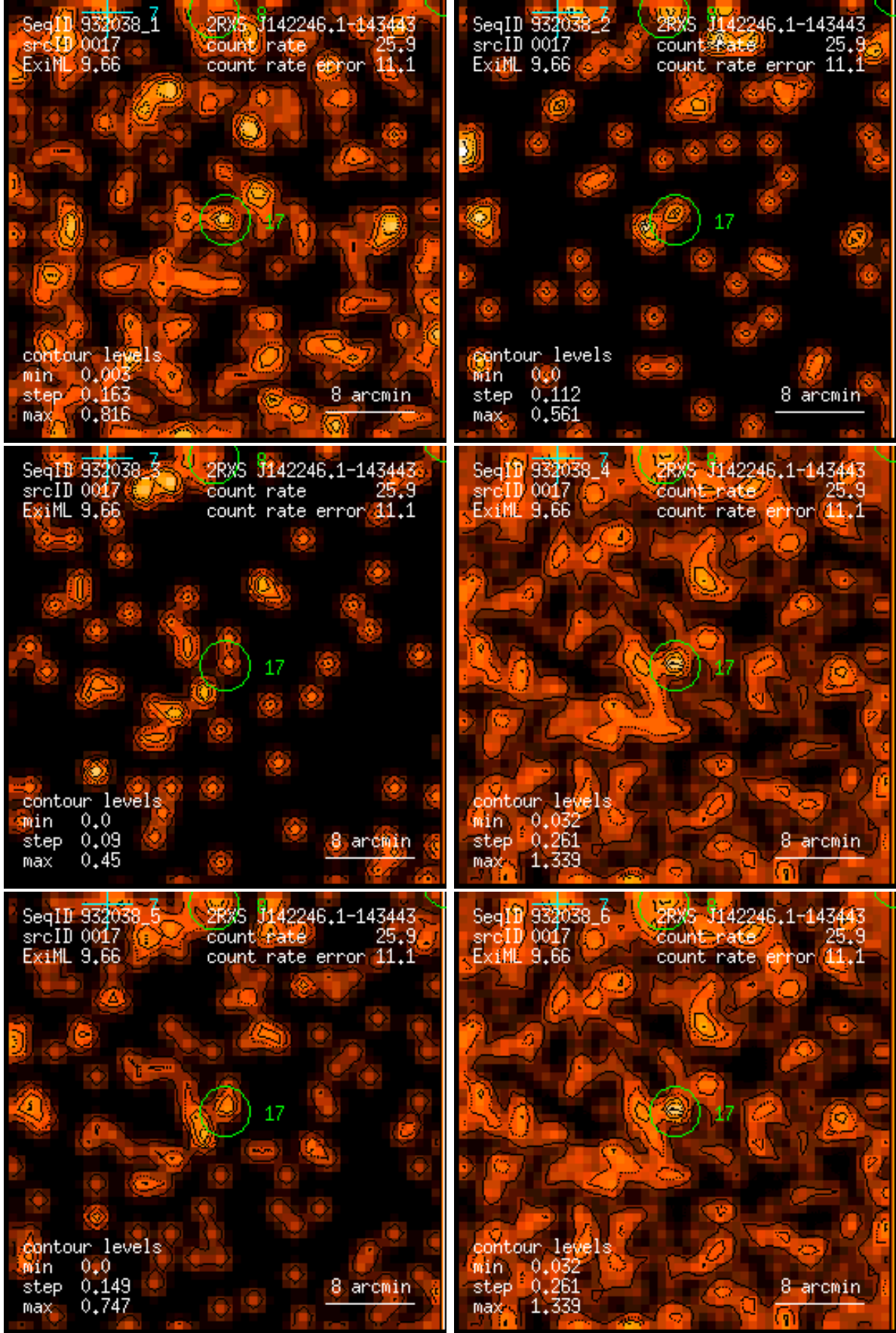
Figure 17: RASS 932038: detection 0017: band rate images, Gaussian filter: (1) PSPC channels 11 – 41, (2) 52 – 90, (3) 91 – 201, (4) 11 – 235, (5) 52 – 201, (6) 11 – 201. Broad band rates in counts/ks. Band rate contour levels in counts/ks/arcmin 2 .
