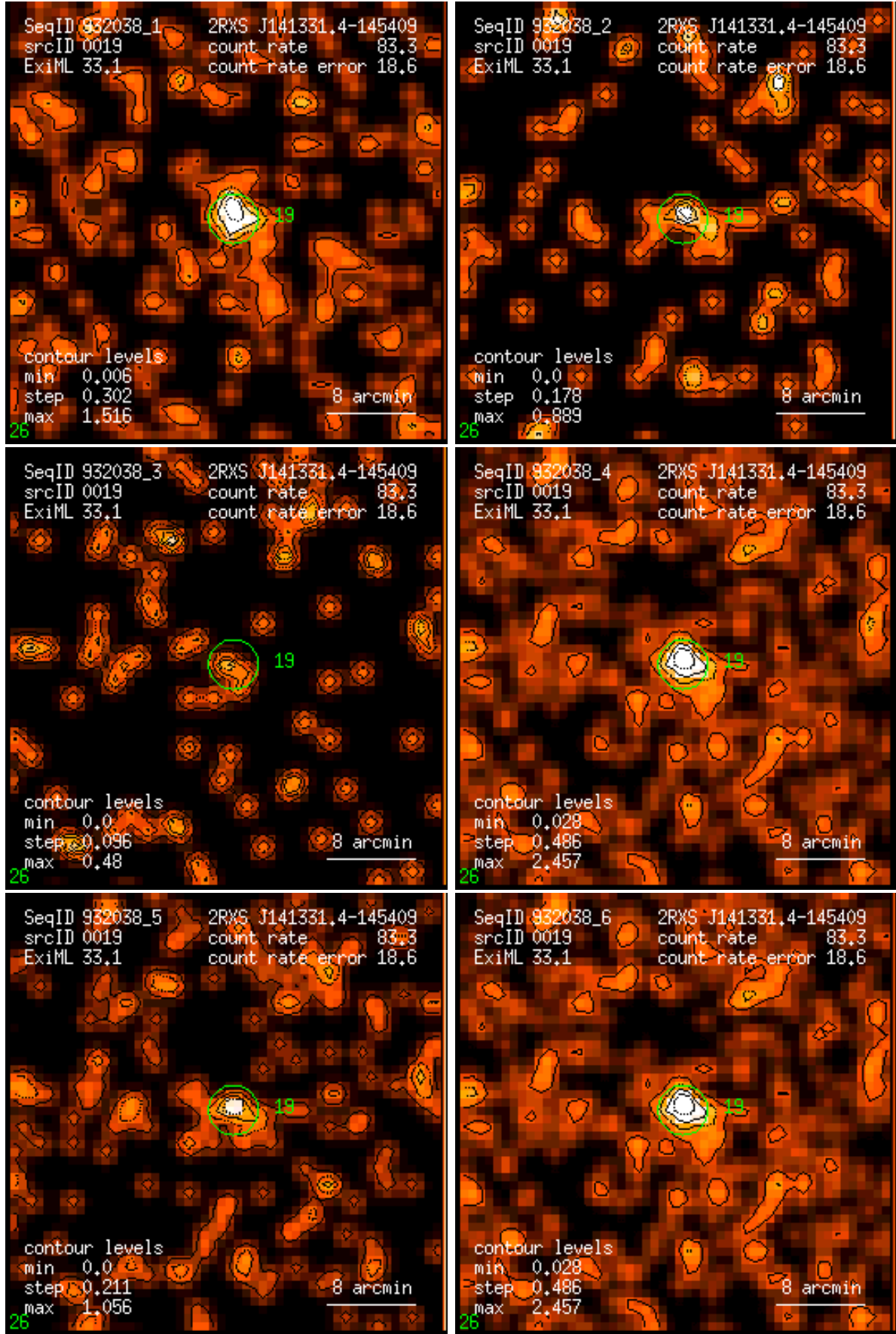
Figure 19: RASS 932038: detection 0019: band rate images, Gaussian filter: (1) PSPC channels 11 – 41, (2) 52 – 90, (3) 91 – 201, (4) 11 – 235, (5) 52 – 201, (6) 11 – 201. Broad band rates in counts/ks. Band rate contour levels in counts/ks/arcmin 2 .
