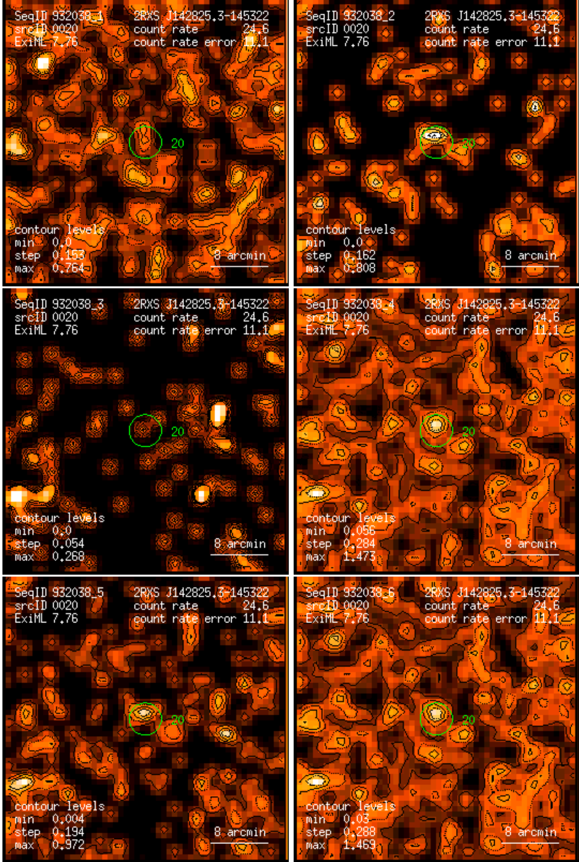
Figure 20: RASS 932038: detection 0020: band rate images, Gaussian filter: (1) PSPC channels 11 – 41, (2) 52 – 90, (3) 91 – 201, (4) 11 – 235, (5) 52 – 201, (6) 11 – 201. Broad band rates in counts/ks. Band rate contour levels in counts/ks/arcmin 2 .
