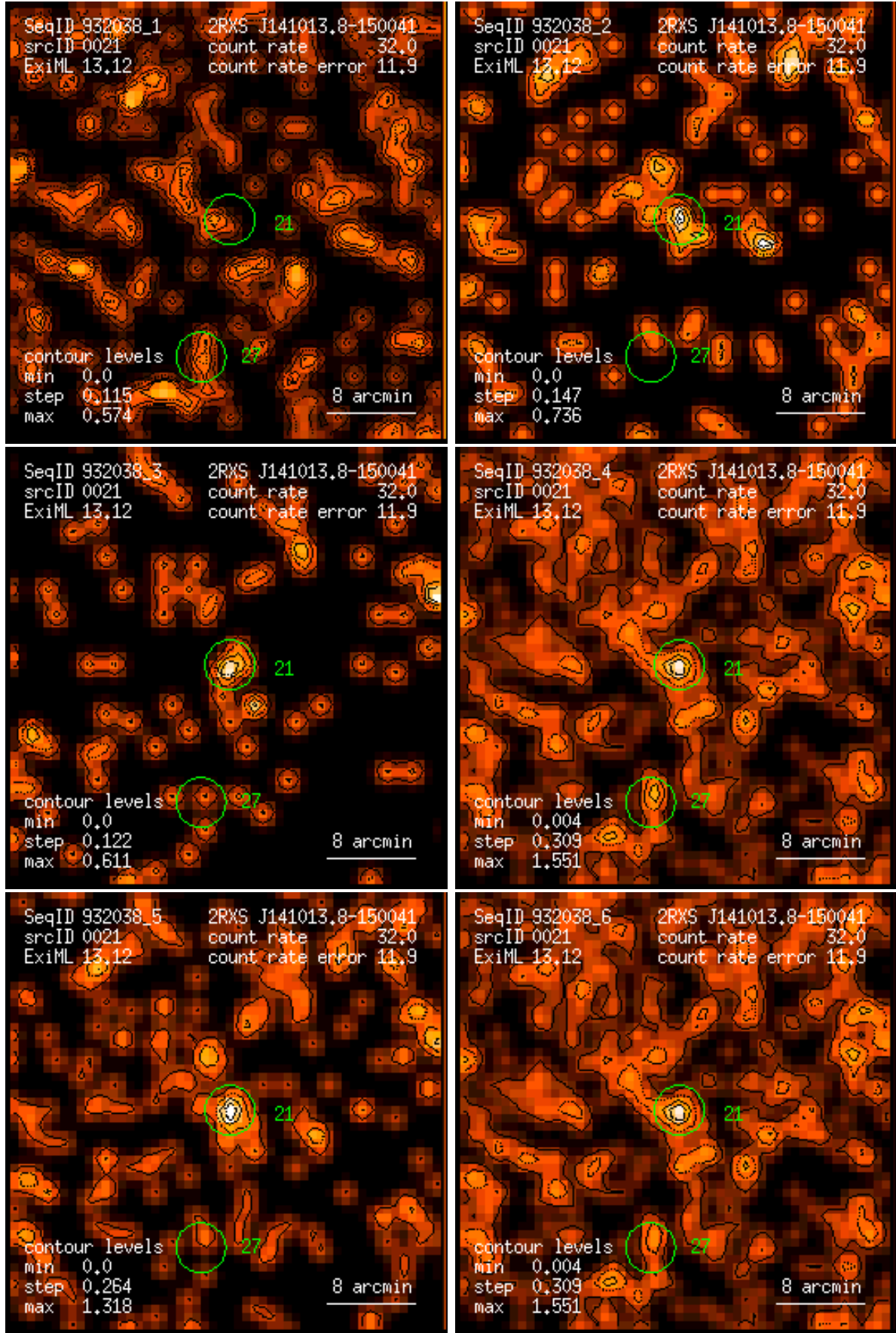
Figure 21: RASS 932038: detection 0021: band rate images, Gaussian filter: (1) PSPC channels 11 – 41, (2) 52 – 90, (3) 91 – 201, (4) 11 – 235, (5) 52 – 201, (6) 11 – 201. Broad band rates in counts/ks. Band rate contour levels in counts/ks/arcmin 2 .
