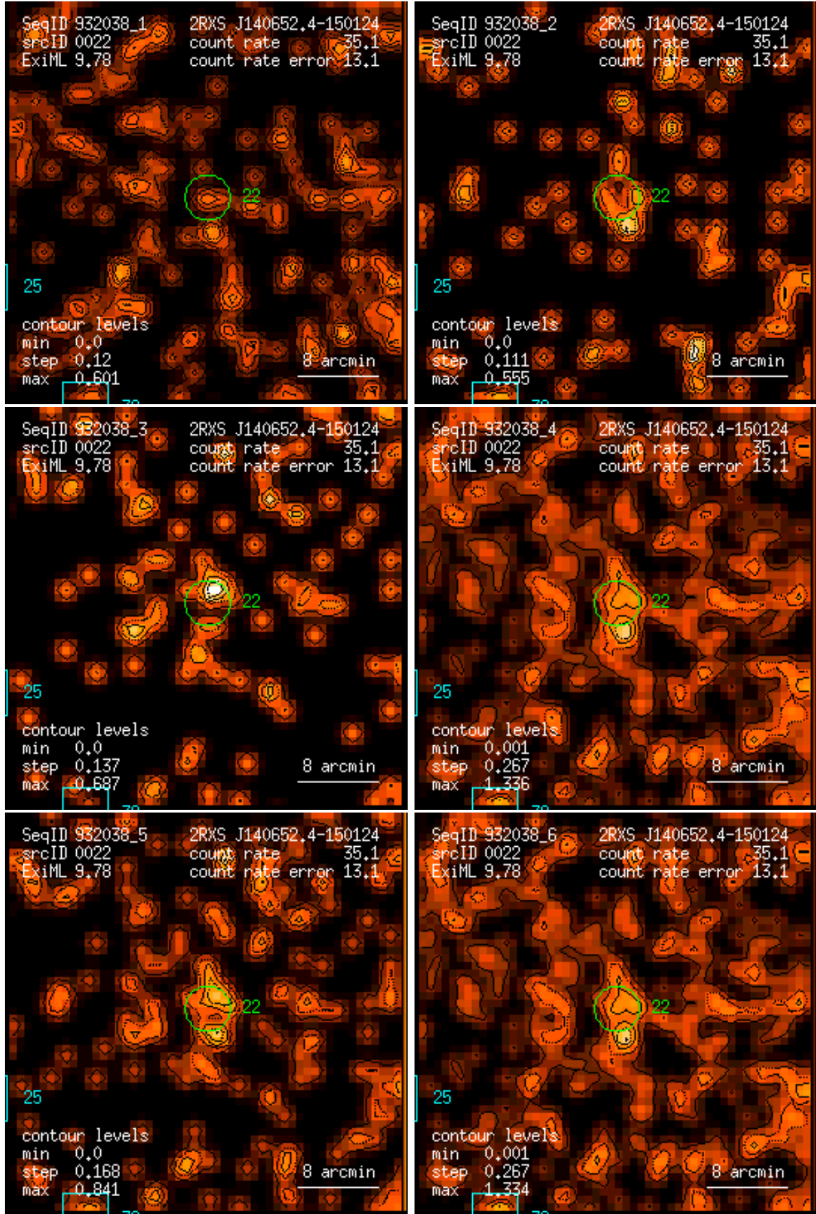
Figure 22: RASS 932038: detection 0022: band rate images, Gaussian filter: (1) PSPC channels 11 – 41, (2) 52 – 90, (3) 91 – 201, (4) 11 – 235, (5) 52 – 201, (6) 11 – 201. Broad band rates in counts/ks. Band rate contour levels in counts/ks/arcmin 2 .
