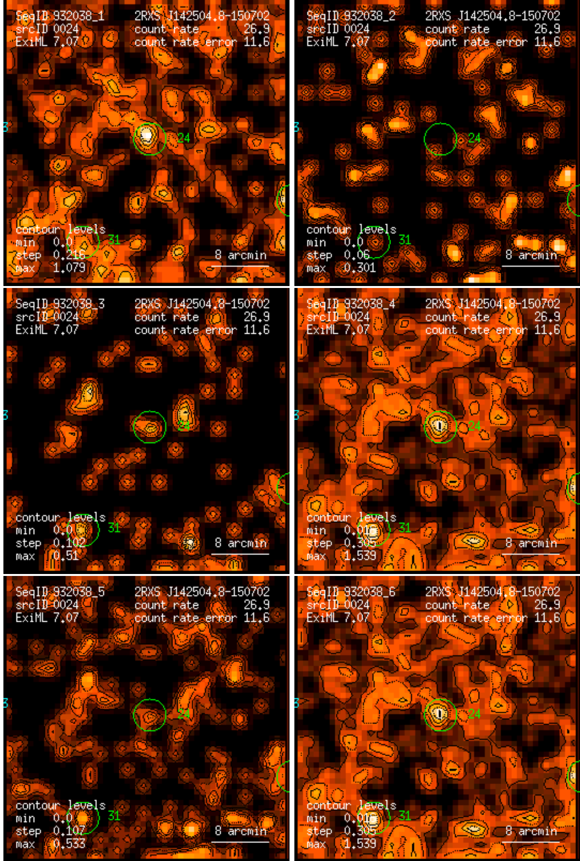
Figure 24: RASS 932038: detection 0024: band rate images, Gaussian filter: (1) PSPC channels 11 – 41, (2) 52 – 90, (3) 91 – 201, (4) 11 – 235, (5) 52 – 201, (6) 11 – 201. Broad band rates in counts/ks. Band rate contour levels in counts/ks/arcmin 2 .
