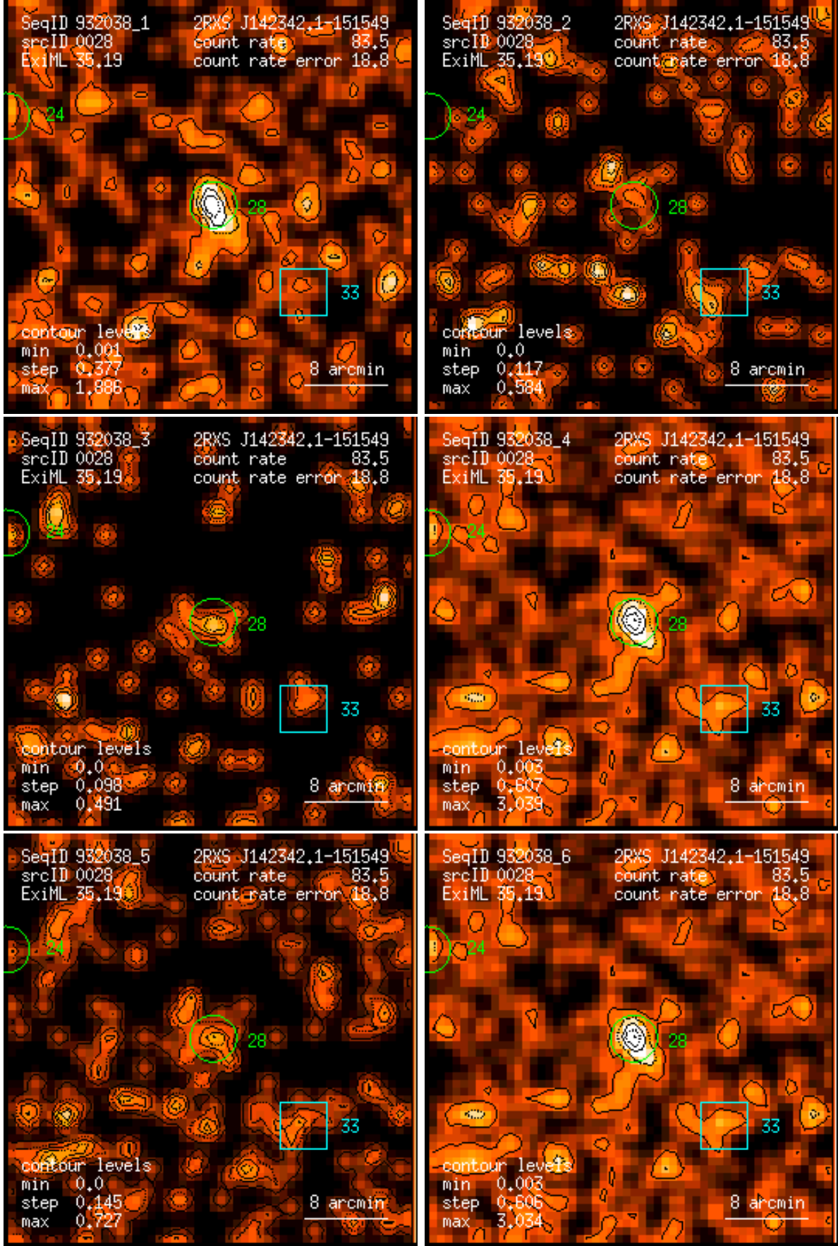
Figure 28: RASS 932038: detection 0028: band rate images, Gaussian filter: (1) PSPC channels 11 – 41, (2) 52 – 90, (3) 91 – 201, (4) 11 – 235, (5) 52 – 201, (6) 11 – 201. Broad band rates in counts/ks. Band rate contour levels in counts/ks/arcmin 2 .
