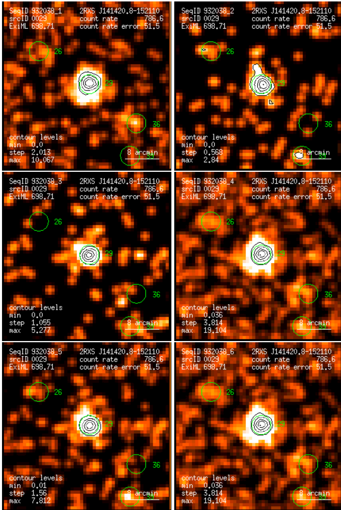
Figure 29: RASS 932038: detection 0029: band rate images, Gaussian filter: (1) PSPC channels 11 – 41, (2) 52 – 90, (3) 91 – 201, (4) 11 – 235, (5) 52 – 201, (6) 11 – 201. Broad band rates in counts/ks. Band rate contour levels in counts/ks/arcmin 2 .
