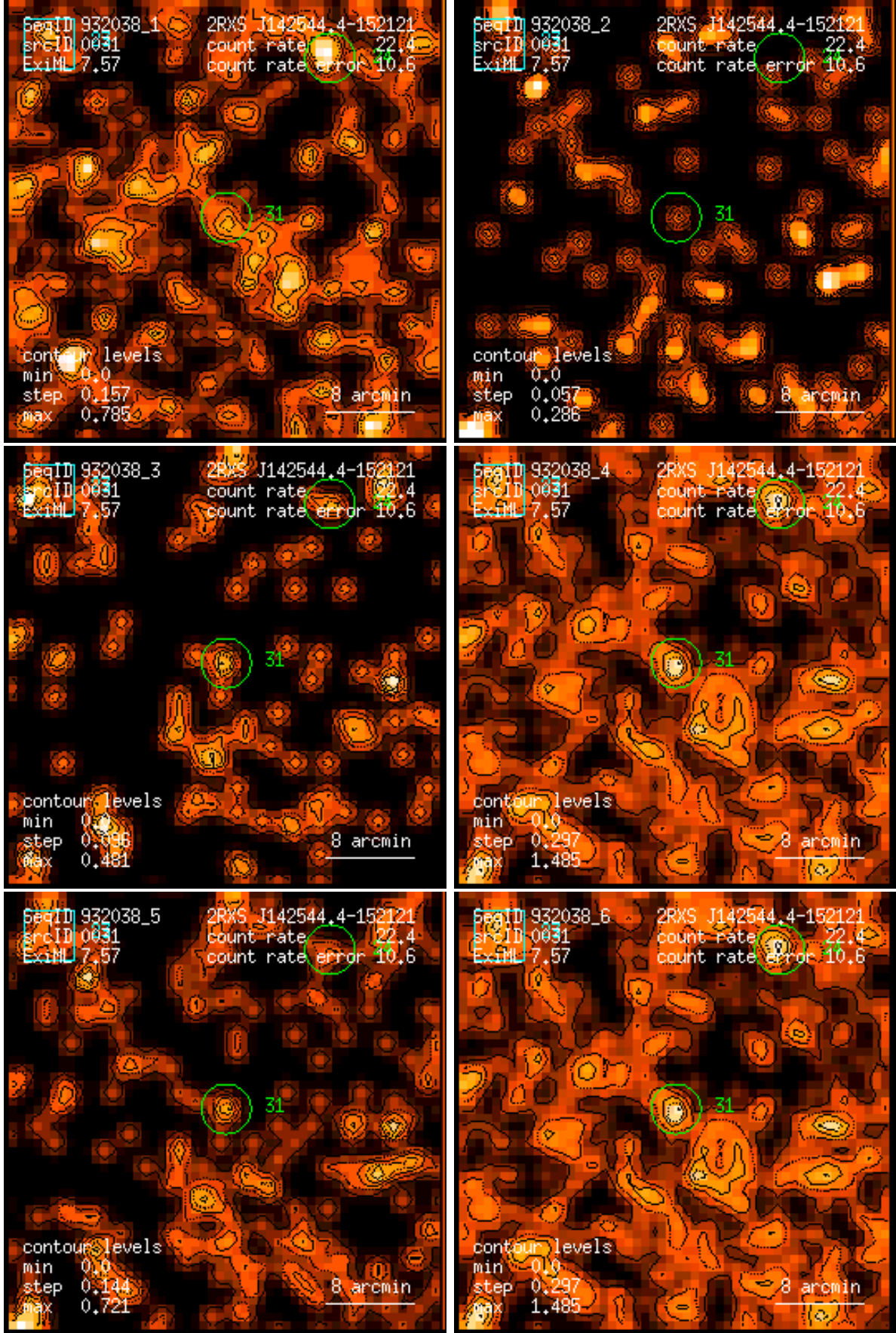
Figure 31: RASS 932038: detection 0031: band rate images, Gaussian filter: (1) PSPC channels 11 – 41, (2) 52 – 90, (3) 91 – 201, (4) 11 – 235, (5) 52 – 201, (6) 11 – 201. Broad band rates in counts/ks. Band rate contour levels in counts/ks/arcmin 2 .
