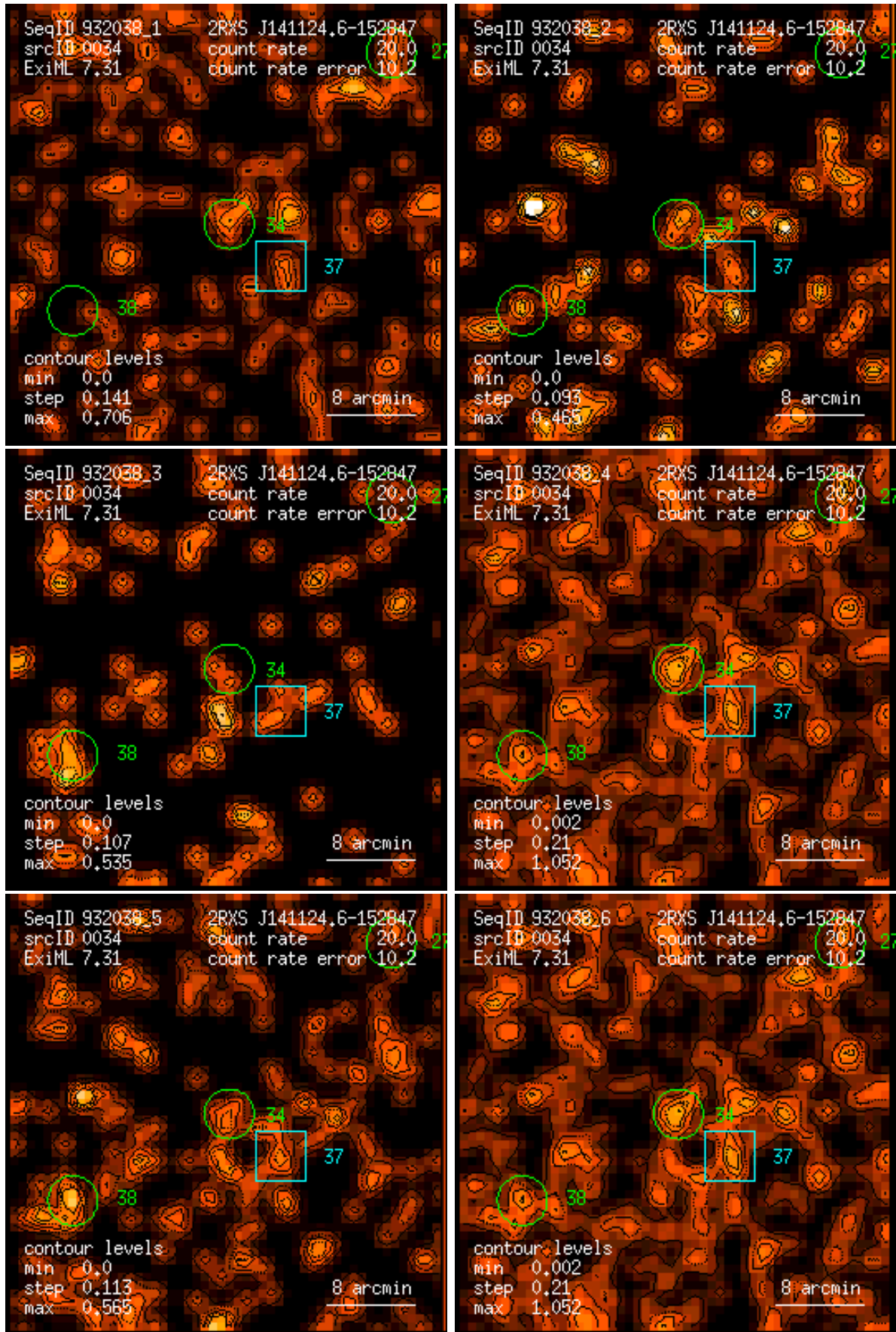
Figure 34: RASS 932038: detection 0034: band rate images, Gaussian filter: (1) PSPC channels 11 – 41, (2) 52 – 90, (3) 91 – 201, (4) 11 – 235, (5) 52 – 201, (6) 11 – 201. Broad band rates in counts/ks. Band rate contour levels in counts/ks/arcmin 2 .
