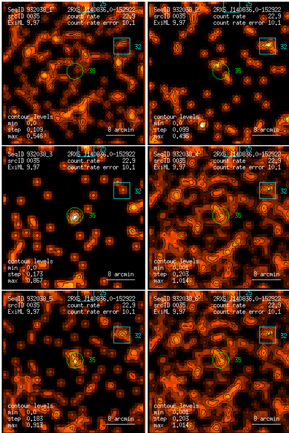
Figure 35: RASS 932038: detection 0035: band rate images, Gaussian filter: (1) PSPC channels 11 – 41, (2) 52 – 90, (3) 91 – 201, (4) 11 – 235, (5) 52 – 201, (6) 11 – 201. Broad band rates in counts/ks. Band rate contour levels in counts/ks/arcmin 2 .
