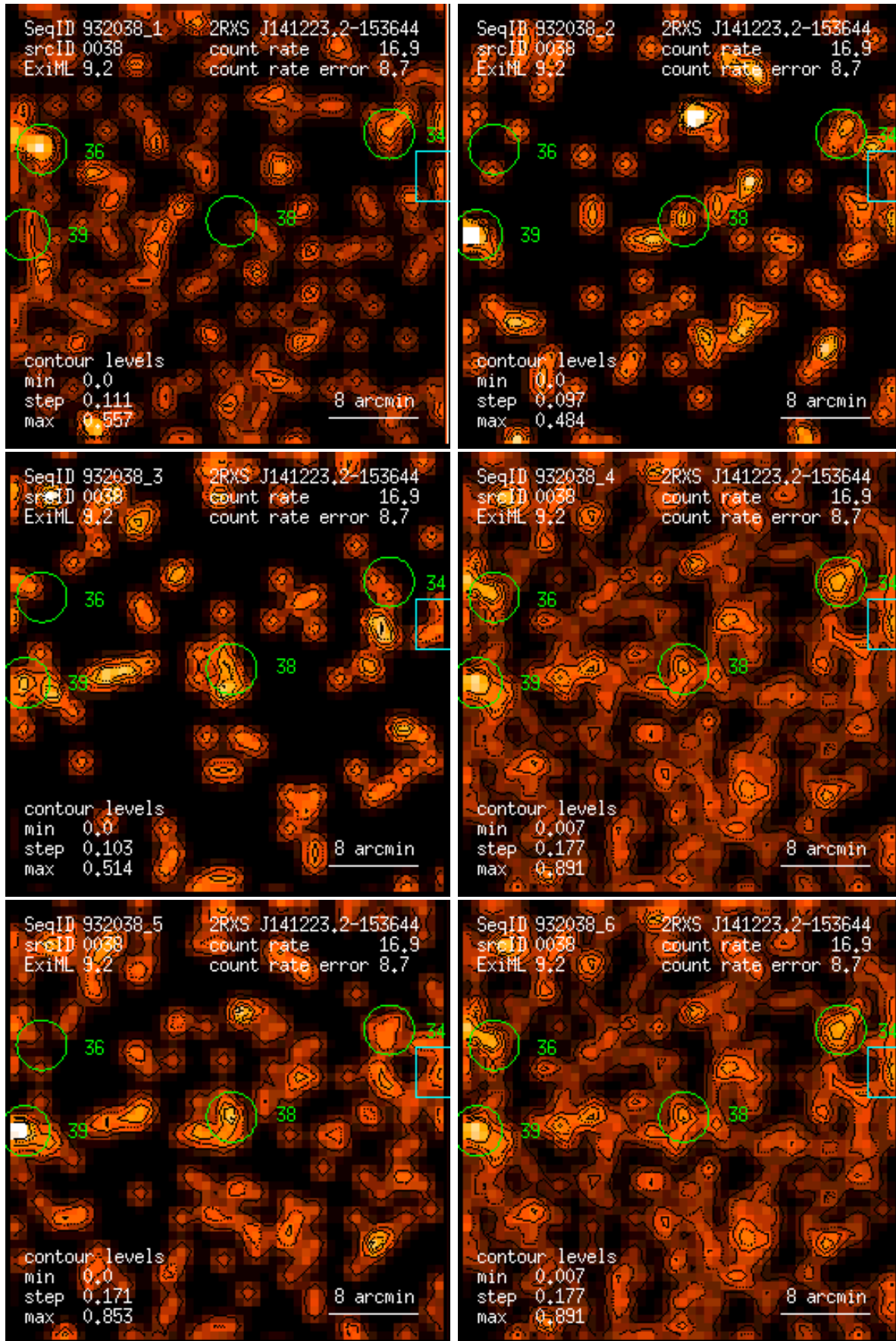
Figure 38: RASS 932038: detection 0038: band rate images, Gaussian filter: (1) PSPC channels 11 – 41, (2) 52 – 90, (3) 91 – 201, (4) 11 – 235, (5) 52 – 201, (6) 11 – 201. Broad band rates in counts/ks. Band rate contour levels in counts/ks/arcmin 2 .
