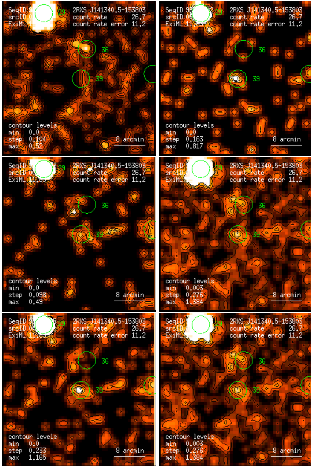
Figure 39: RASS 932038: detection 0039: band rate images, Gaussian filter: (1) PSPC channels 11 – 41, (2) 52 – 90, (3) 91 – 201, (4) 11 – 235, (5) 52 – 201, (6) 11 – 201. Broad band rates in counts/ks. Band rate contour levels in counts/ks/arcmin 2 .
