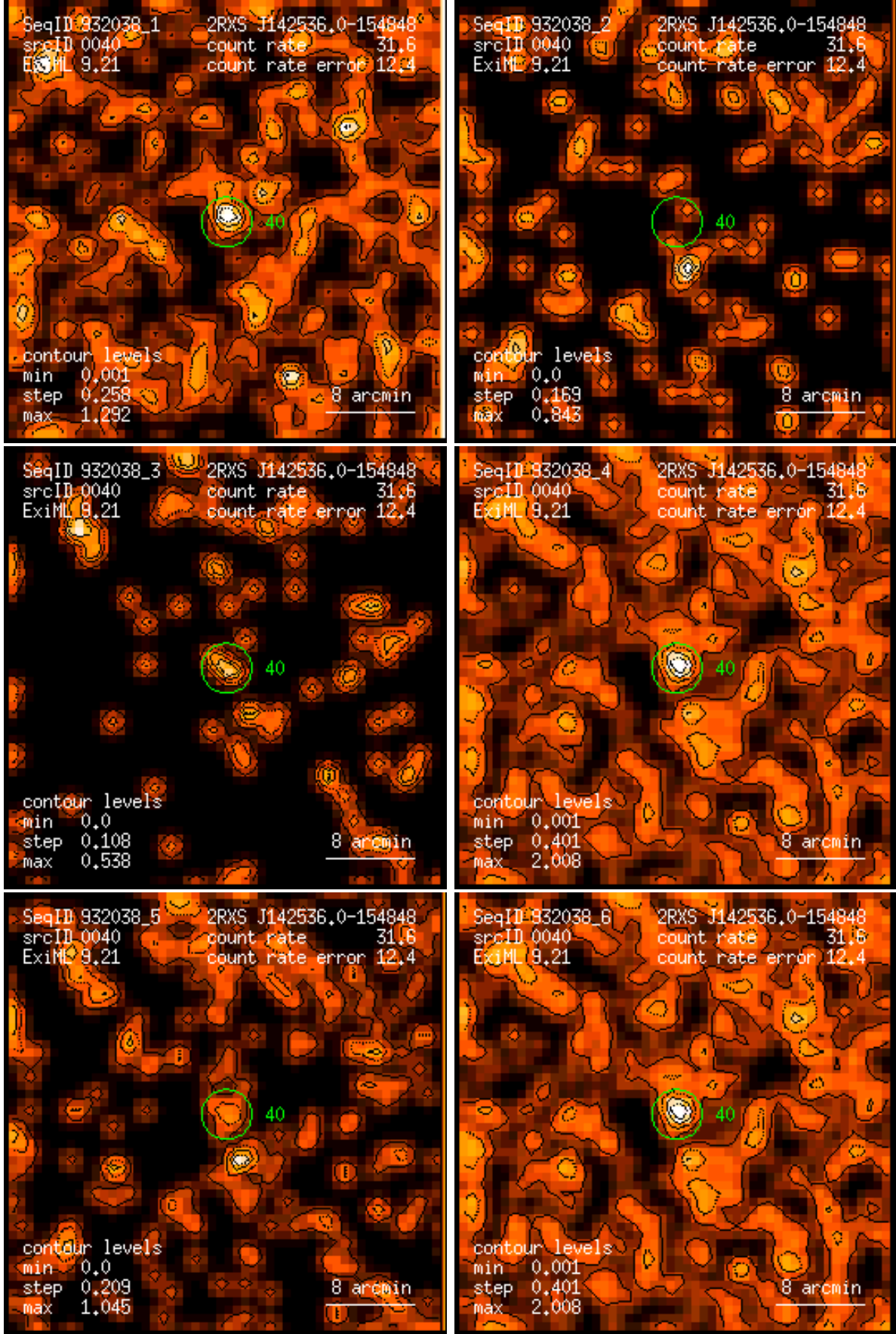
Figure 40: RASS 932038: detection 0040: band rate images, Gaussian filter: (1) PSPC channels 11 – 41, (2) 52 – 90, (3) 91 – 201, (4) 11 – 235, (5) 52 – 201, (6) 11 – 201. Broad band rates in counts/ks. Band rate contour levels in counts/ks/arcmin 2 .
