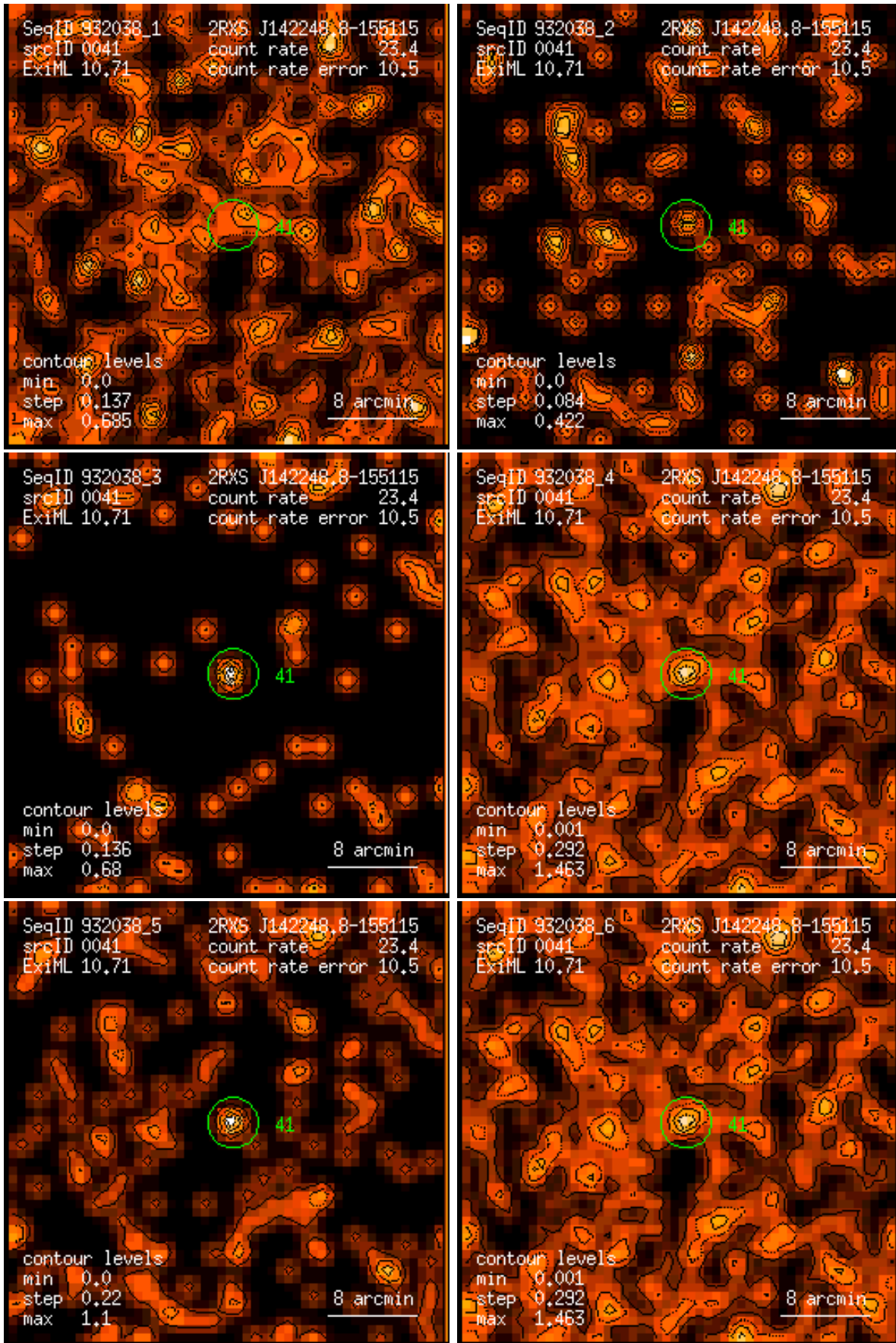
Figure 41: RASS 932038: detection 0041: band rate images, Gaussian filter: (1) PSPC channels 11 – 41, (2) 52 – 90, (3) 91 – 201, (4) 11 – 235, (5) 52 – 201, (6) 11 – 201. Broad band rates in counts/ks. Band rate contour levels in counts/ks/arcmin 2 .
