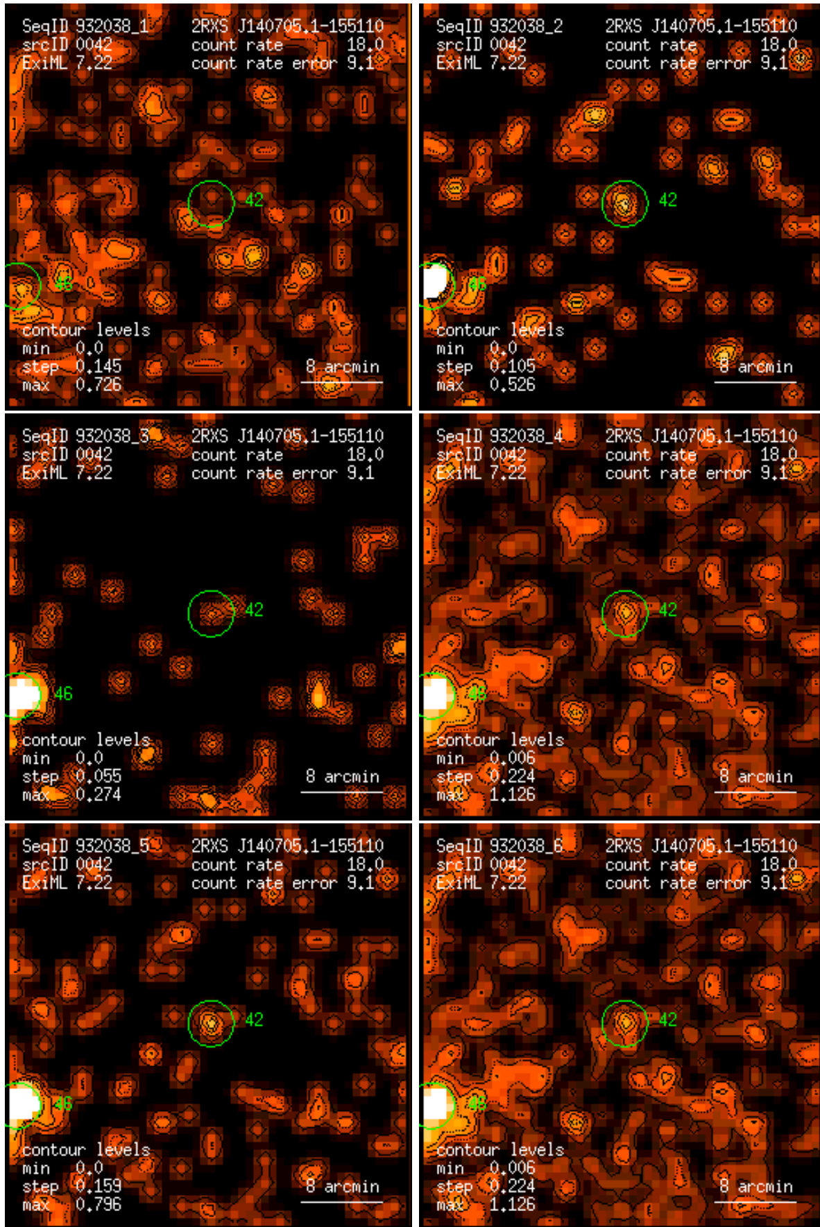
Figure 42: RASS 932038: detection 0042: band rate images, Gaussian filter: (1) PSPC channels 11 – 41, (2) 52 – 90, (3) 91 – 201, (4) 11 – 235, (5) 52 – 201, (6) 11 – 201. Broad band rates in counts/ks. Band rate contour levels in counts/ks/arcmin 2 .
