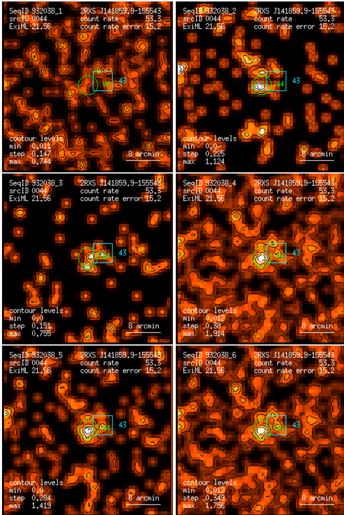
Figure 44: RASS 932038: detection 0044: band rate images, Gaussian filter: (1) PSPC channels 11 – 41, (2) 52 – 90, (3) 91 – 201, (4) 11 – 235, (5) 52 – 201, (6) 11 – 201. Broad band rates in counts/ks. Band rate contour levels in counts/ks/arcmin 2 .
