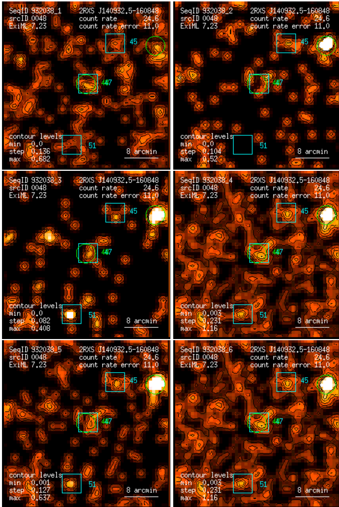
Figure 48: RASS 932038: detection 0048: band rate images, Gaussian filter: (1) PSPC channels 11 – 41, (2) 52 – 90, (3) 91 – 201, (4) 11 – 235, (5) 52 – 201, (6) 11 – 201. Broad band rates in counts/ks. Band rate contour levels in counts/ks/arcmin 2 .
