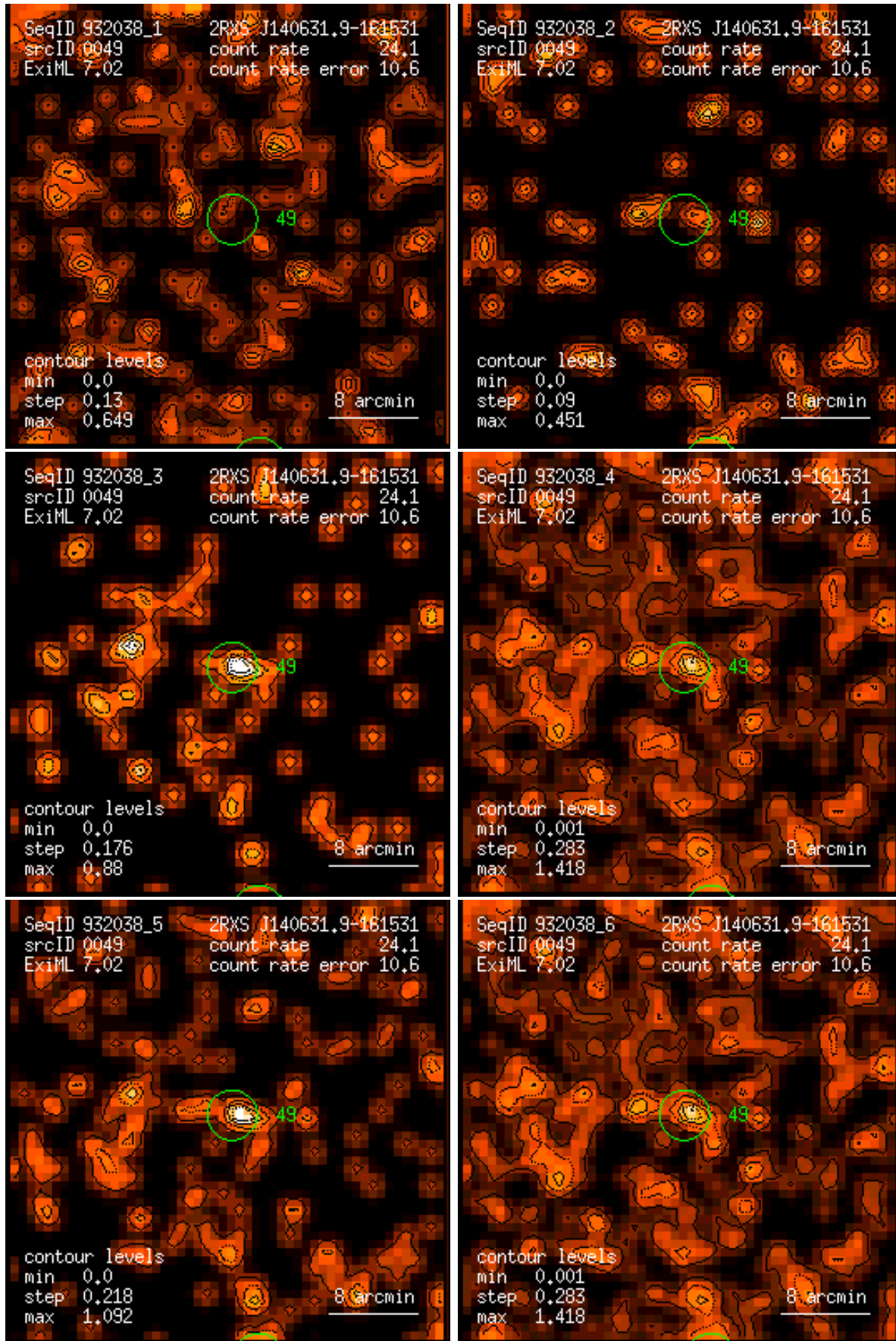
Figure 49: RASS 932038: detection 0049: band rate images, Gaussian filter: (1) PSPC channels 11 – 41, (2) 52 – 90, (3) 91 – 201, (4) 11 – 235, (5) 52 – 201, (6) 11 – 201. Broad band rates in counts/ks. Band rate contour levels in counts/ks/arcmin 2 .
