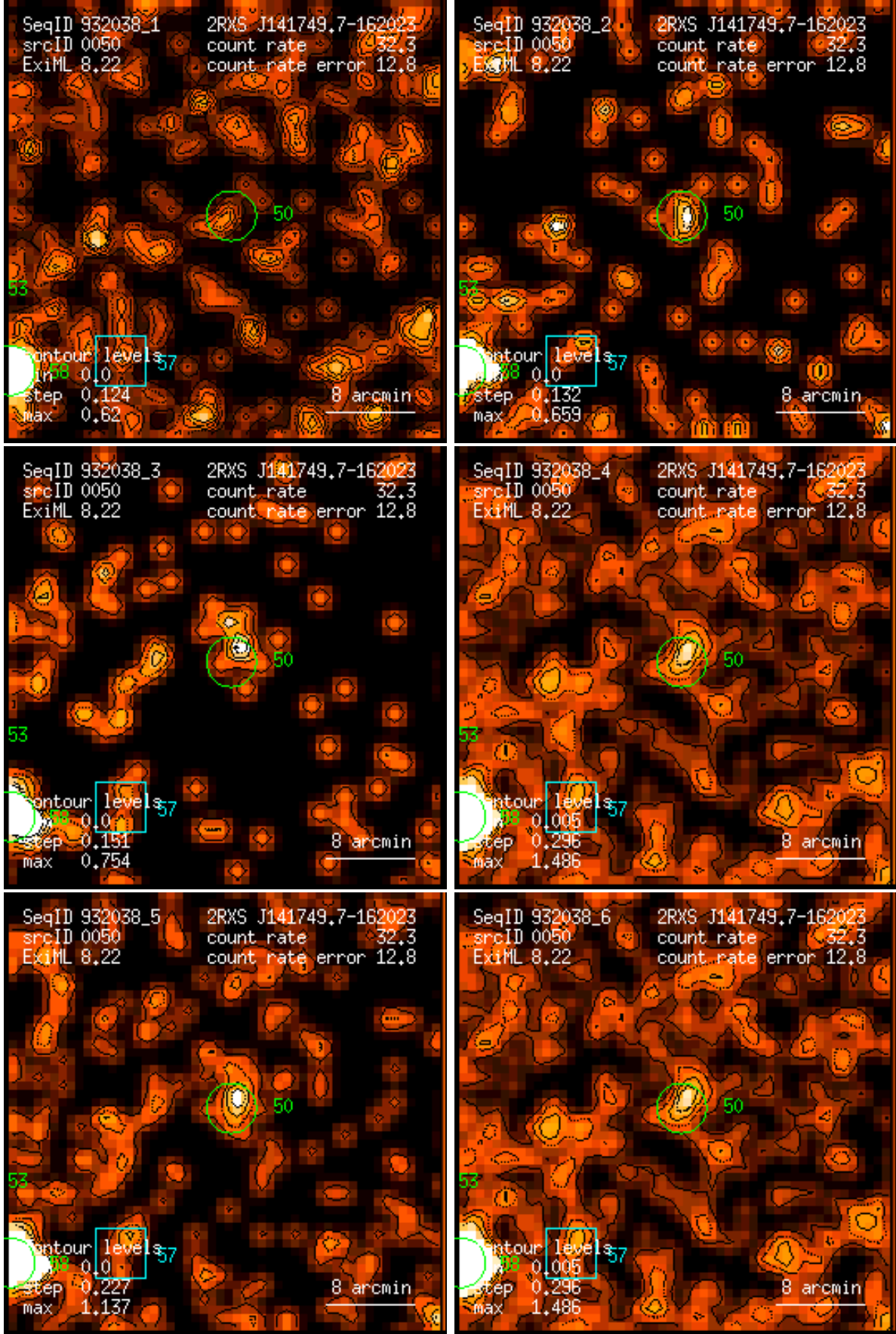
Figure 50: RASS 932038: detection 0050: band rate images, Gaussian filter: (1) PSPC channels 11 – 41, (2) 52 – 90, (3) 91 – 201, (4) 11 – 235, (5) 52 – 201, (6) 11 – 201. Broad band rates in counts/ks. Band rate contour levels in counts/ks/arcmin 2 .
