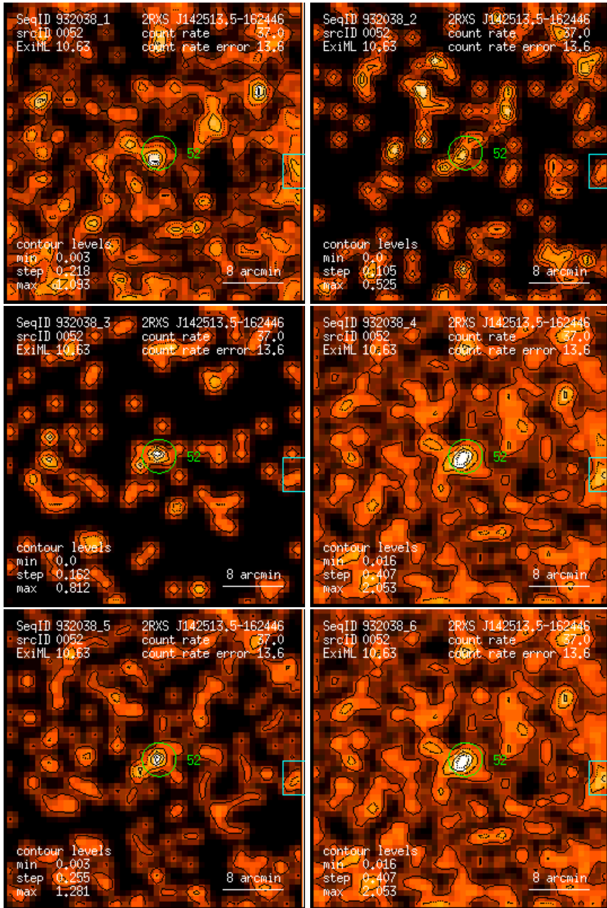
Figure 52: RASS 932038: detection 0052: band rate images, Gaussian filter: (1) PSPC channels 11 – 41, (2) 52 – 90, (3) 91 – 201, (4) 11 – 235, (5) 52 – 201, (6) 11 – 201. Broad band rates in counts/ks. Band rate contour levels in counts/ks/arcmin 2 .
