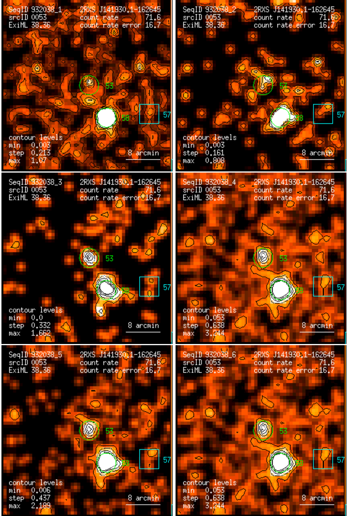
Figure 53: RASS 932038: detection 0053: band rate images, Gaussian filter: (1) PSPC channels 11 – 41, (2) 52 – 90, (3) 91 – 201, (4) 11 – 235, (5) 52 – 201, (6) 11 – 201. Broad band rates in counts/ks. Band rate contour levels in counts/ks/arcmin 2 .
