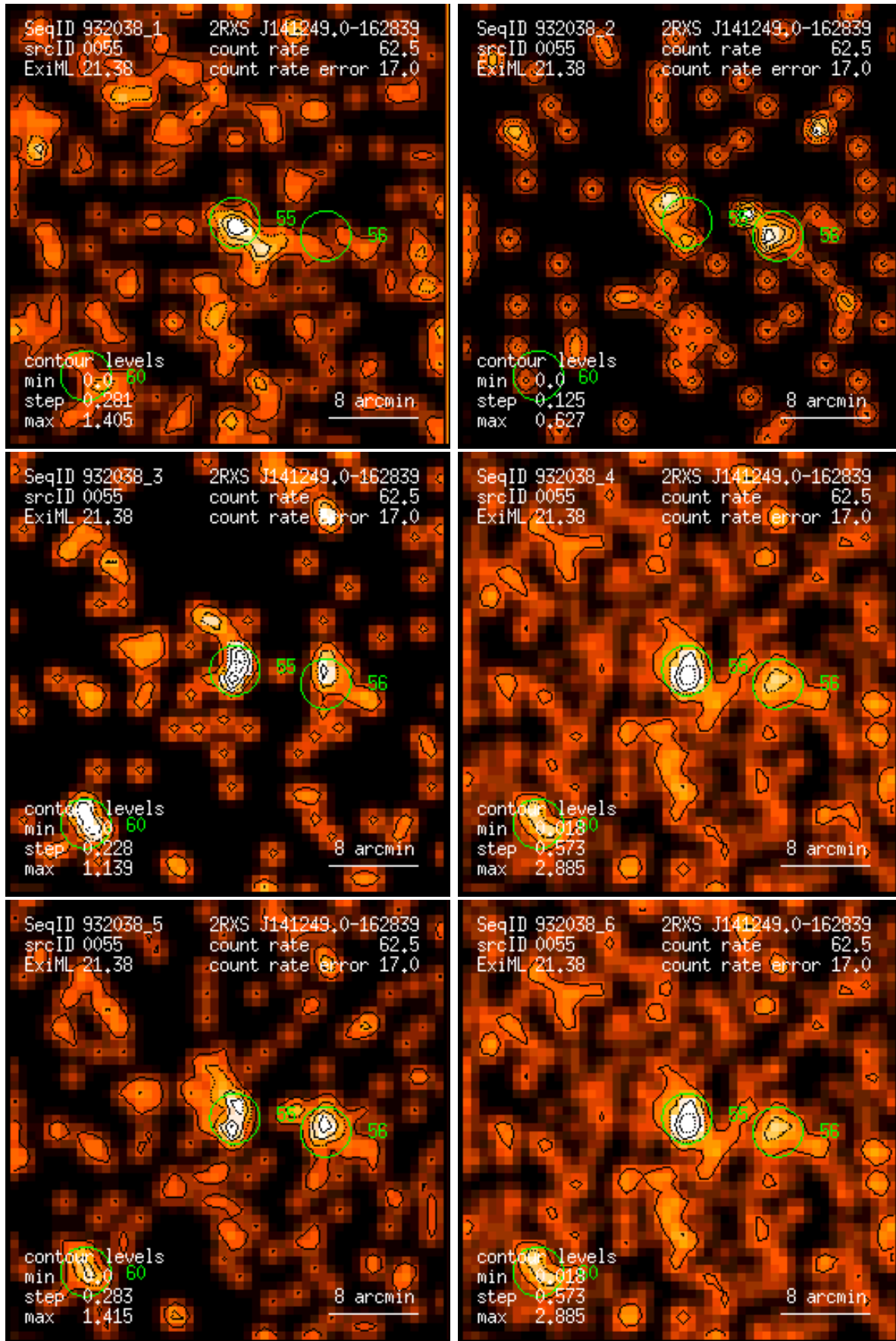
Figure 55: RASS 932038: detection 0055: band rate images, Gaussian filter: (1) PSPC channels 11 – 41, (2) 52 – 90, (3) 91 – 201, (4) 11 – 235, (5) 52 – 201, (6) 11 – 201. Broad band rates in counts/ks. Band rate contour levels in counts/ks/arcmin 2 .
