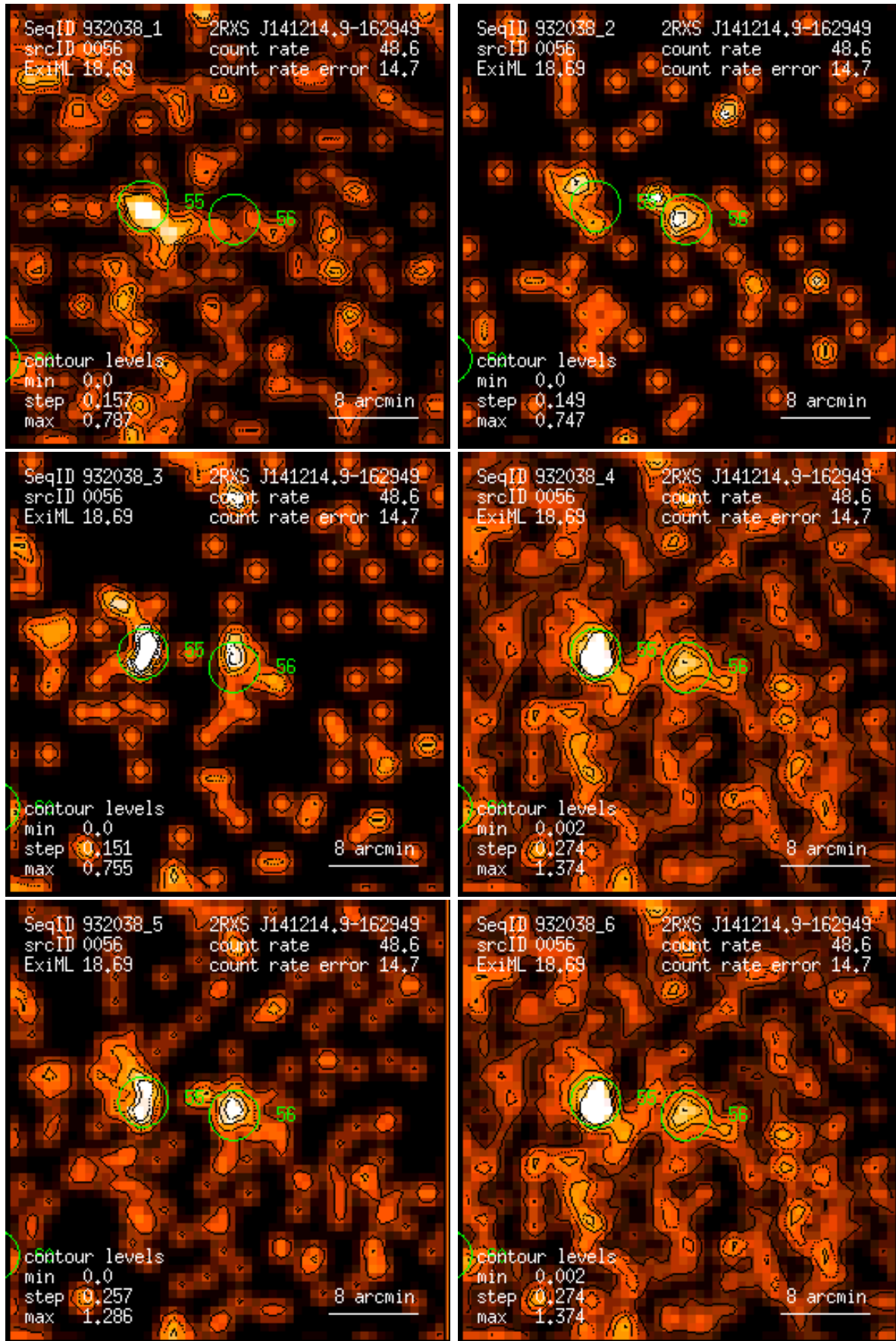
Figure 56: RASS 932038: detection 0056: band rate images, Gaussian filter: (1) PSPC channels 11 – 41, (2) 52 – 90, (3) 91 – 201, (4) 11 – 235, (5) 52 – 201, (6) 11 – 201. Broad band rates in counts/ks. Band rate contour levels in counts/ks/arcmin 2 .
