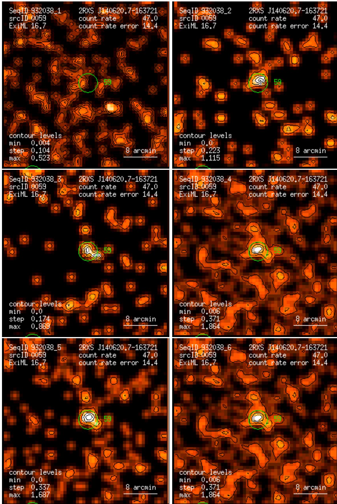
Figure 59: RASS 932038: detection 0059: band rate images, Gaussian filter: (1) PSPC channels 11 – 41, (2) 52 – 90, (3) 91 – 201, (4) 11 – 235, (5) 52 – 201, (6) 11 – 201. Broad band rates in counts/ks. Band rate contour levels in counts/ks/arcmin 2 .
