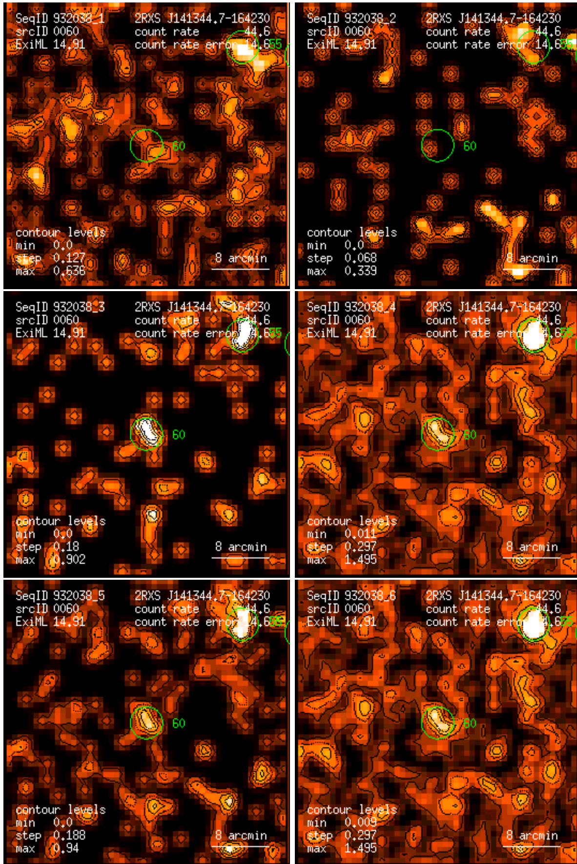
Figure 60: RASS 932038: detection 0060: band rate images, Gaussian filter: (1) PSPC channels 11 – 41, (2) 52 – 90, (3) 91 – 201, (4) 11 – 235, (5) 52 – 201, (6) 11 – 201. Broad band rates in counts/ks. Band rate contour levels in counts/ks/arcmin 2 .
