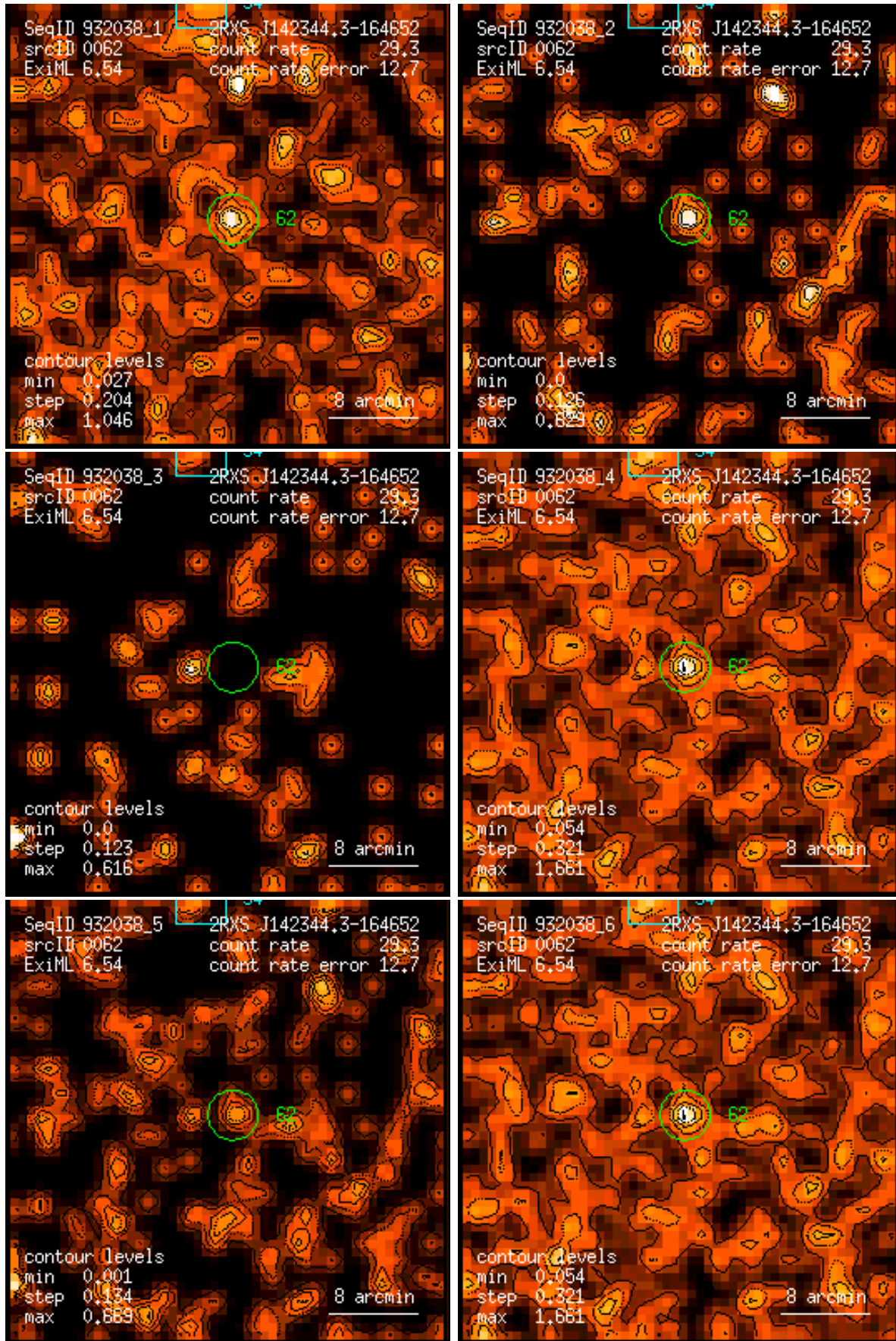
Figure 62: RASS 932038: detection 0062: band rate images, Gaussian filter: (1) PSPC channels 11 – 41, (2) 52 – 90, (3) 91 – 201, (4) 11 – 235, (5) 52 – 201, (6) 11 – 201. Broad band rates in counts/ks. Band rate contour levels in counts/ks/arcmin 2 .
