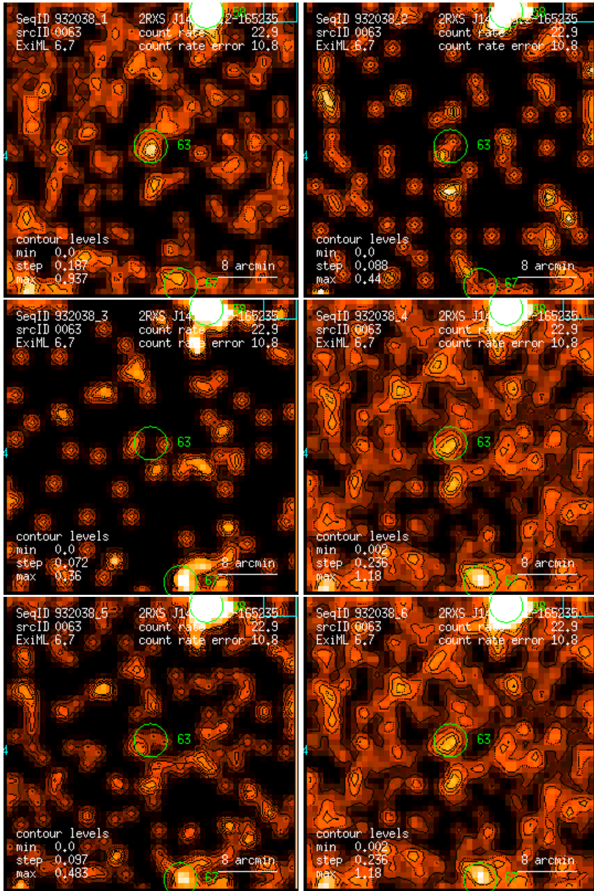
Figure 63: RASS 932038: detection 0063: band rate images, Gaussian filter: (1) PSPC channels 11 – 41, (2) 52 – 90, (3) 91 – 201, (4) 11 – 235, (5) 52 – 201, (6) 11 – 201. Broad band rates in counts/ks. Band rate contour levels in counts/ks/arcmin 2 .
