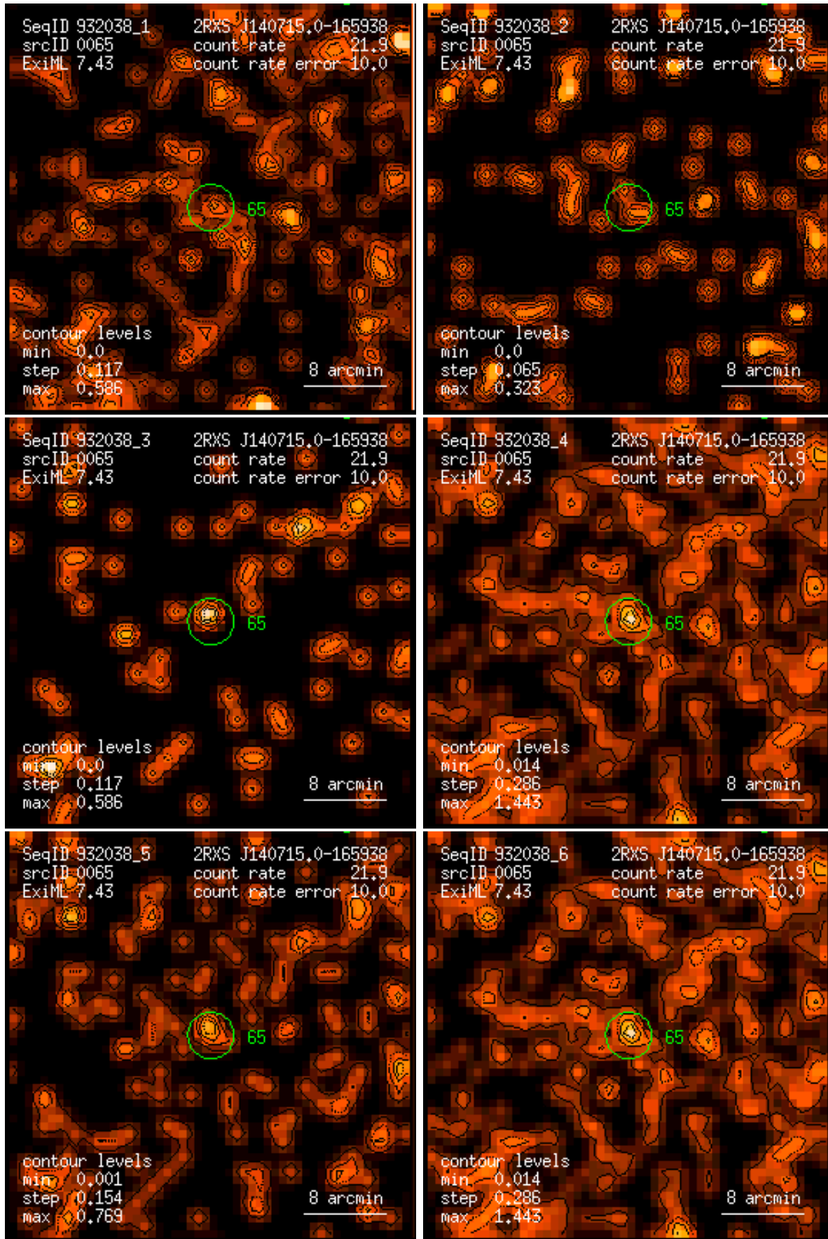
Figure 65: RASS 932038: detection 0065: band rate images, Gaussian filter: (1) PSPC channels 11 – 41, (2) 52 – 90, (3) 91 – 201, (4) 11 – 235, (5) 52 – 201, (6) 11 – 201. Broad band rates in counts/ks. Band rate contour levels in counts/ks/arcmin 2 .
